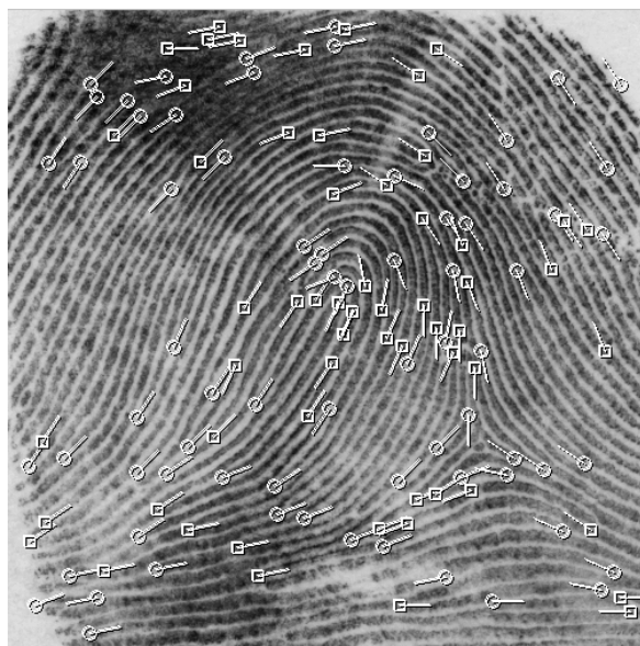
Figure 40. Minutiae results.
