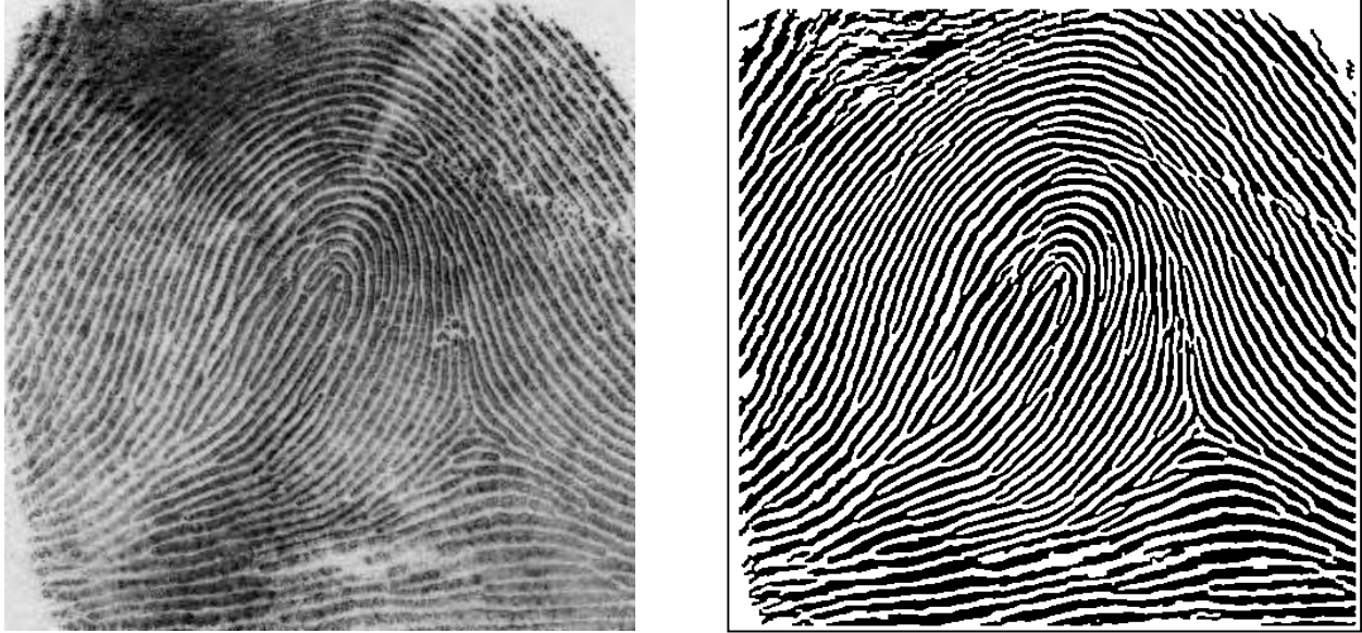
Figure 28. Binarization results
