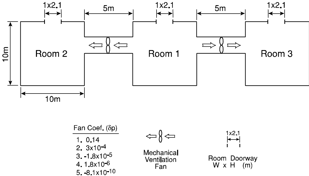
Figure 6. Plan diagram of the geometry used in the mechanical ventilation and HCl deposition calculation.
