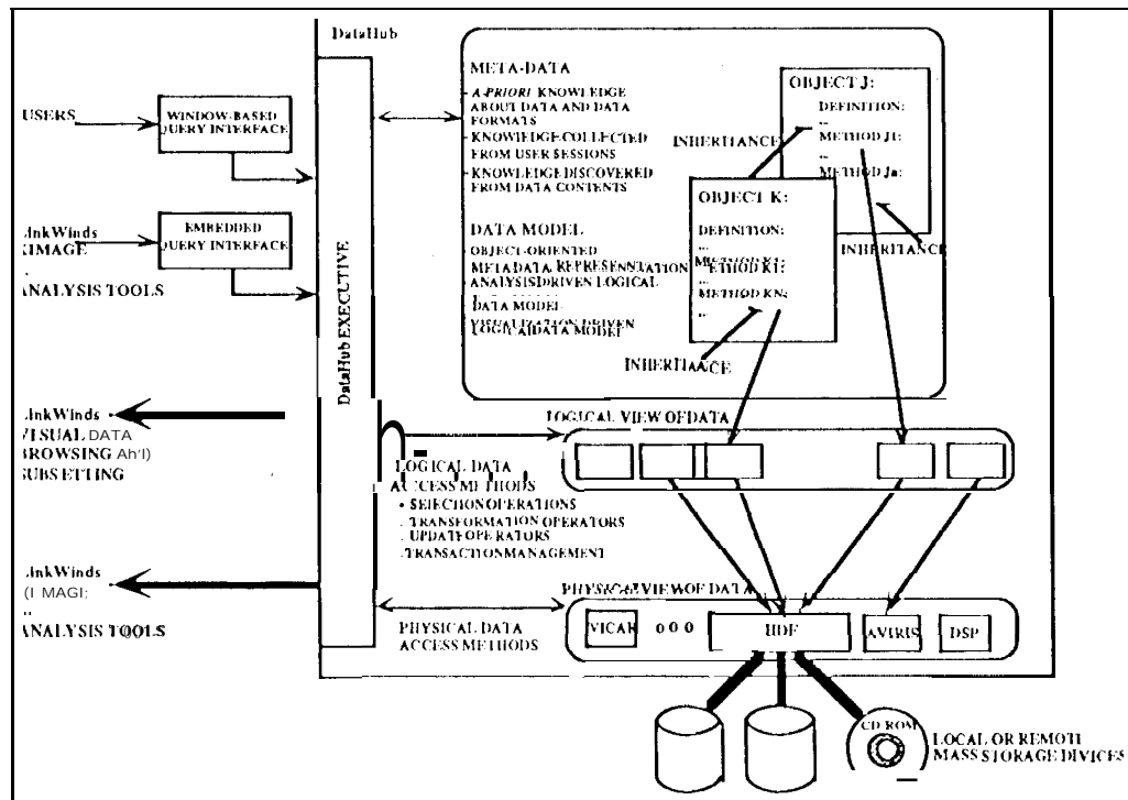
Figure 1 -- Functional Architecture
