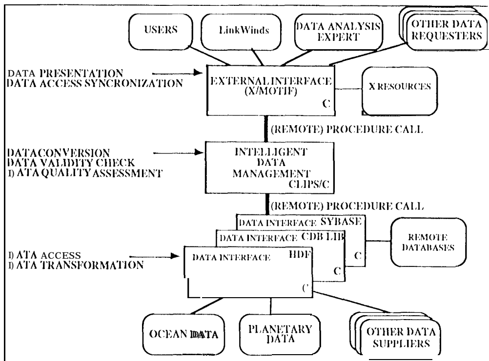
Figure 2 -- Software Architecture
