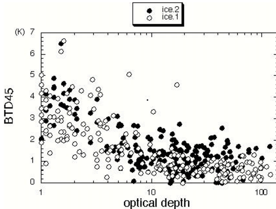
Figure 3. Same as Figure 2, except for clouds identified as ice phase only.
