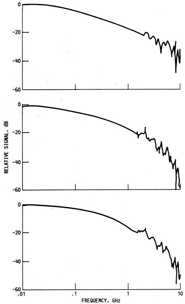
Fig. 4. Normalized frequency response of typical detectors. (a) 1 \mu\text{m} x 1 \mu\text{m} ; (b) 2 \mu\text{m} x 2 \mu\text{m} ; (c) 2 \mu\text{m} x 2 \mu\text{m} .
