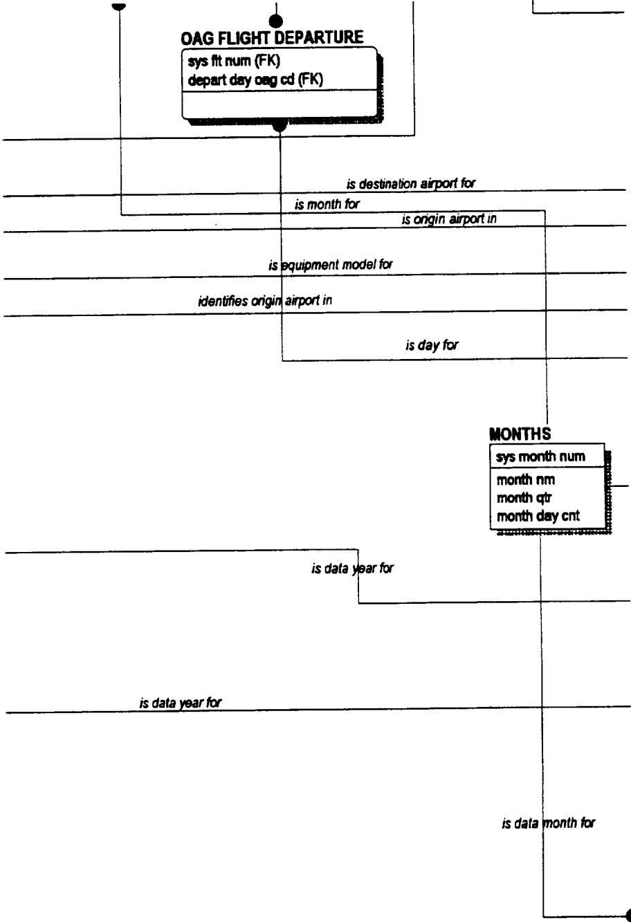
Figure A-2. QRS Database Entity-Relationship Diagram (Con't.)
