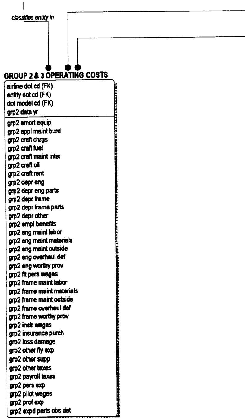
Figure A-2. QRS Database Entity-Relationship Diagram (Con't.)
