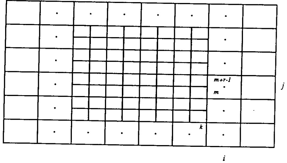
FIG. 8. The difference scheme is modified at a coarse cell abutting a fine grid.
