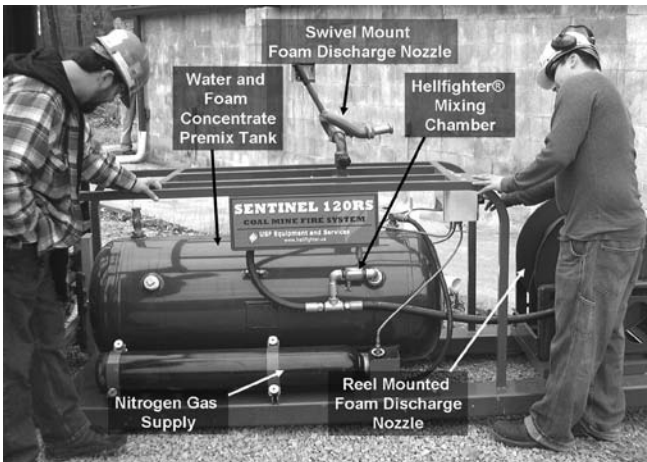
Figure 9 —USF Sentinel® unit used during crib block fire Test 4.
