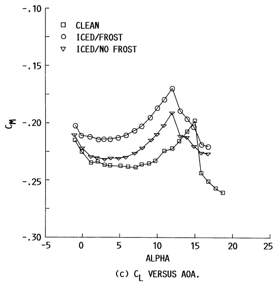
FIGURE 14. - ICE SHAPE TRACINGS AND FORCE BALANCE MEASUREMENTS FOR RUN NUMBER 12.
