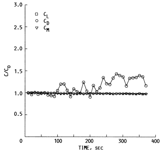
(d) RATIO OF FORCED COEFFICIENTS/FORCE COEFFICIENT OF CLEAN AIRFOIL VERSUS TIME.
