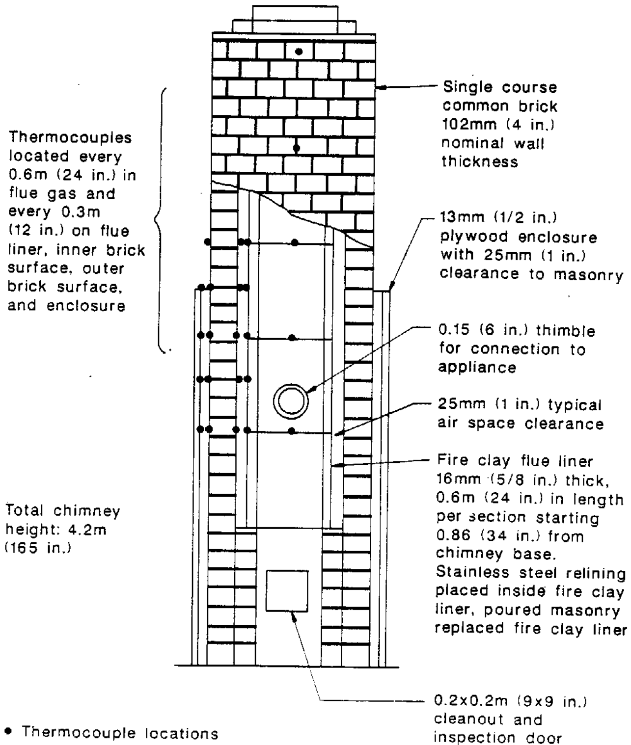
Figure 1: Masonry Chimney Design and Instrumentation
