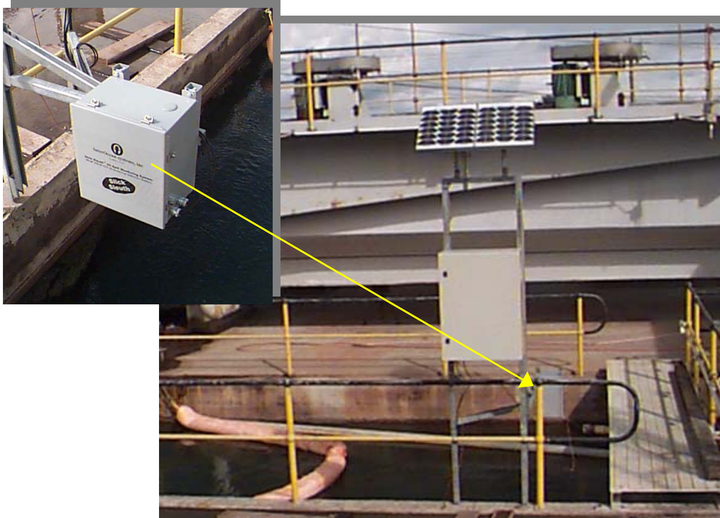
Autonomous Spill Detection Sensor w/DC Power System photo courtesy of Shell Australia
