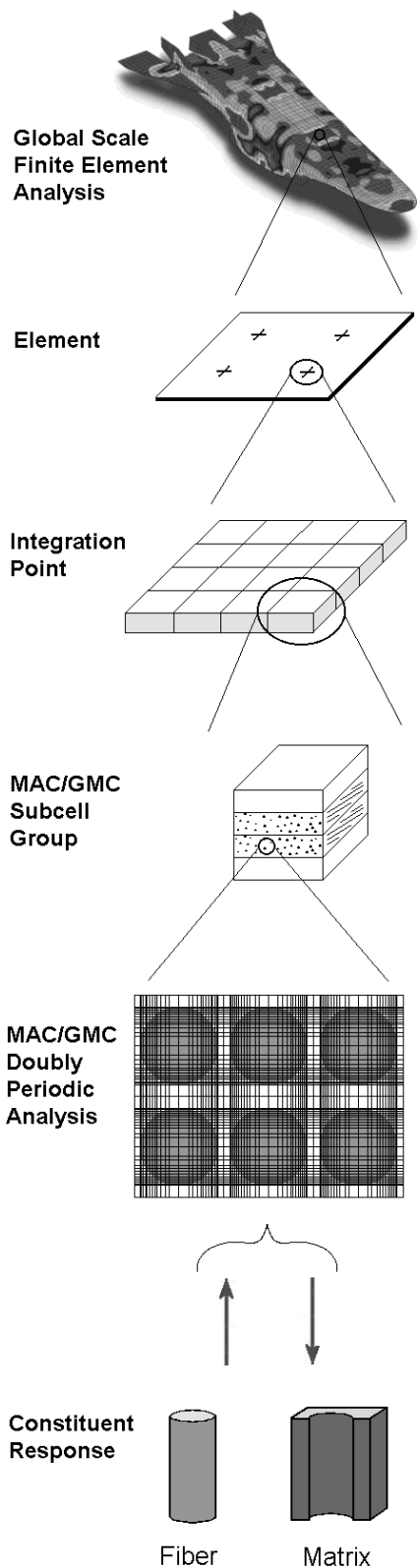
Fig. 12. Illustration of a multi-scale approach to modeling woven composite materials and structures.
