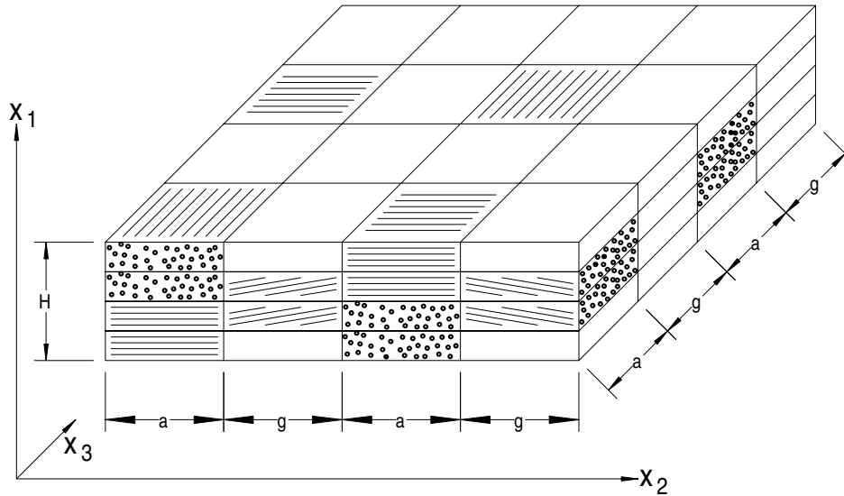
Fig. 2. MAC/GMC repeating unit cell used to represent a plain weave composite.
