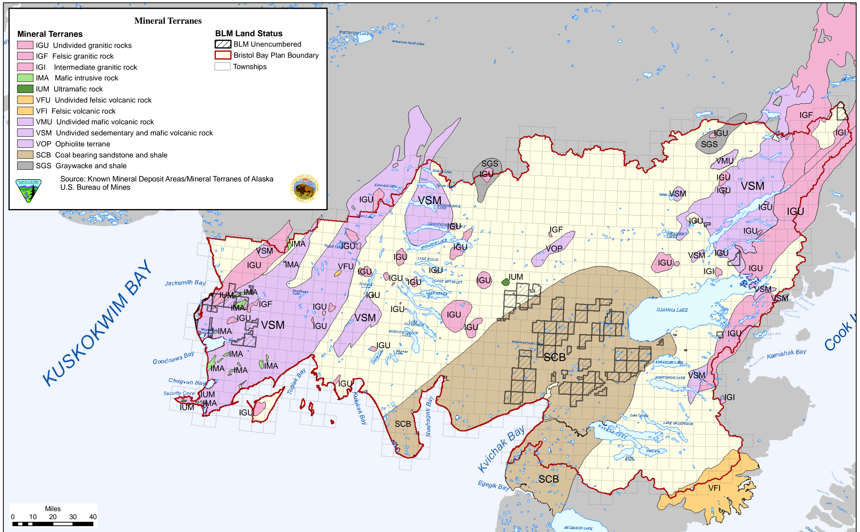
Figure 3.77 Mineral Terranes
