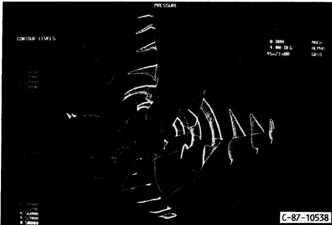
FIGURE 13. - UNSTEADY THREE DIMENSIONAL EULER CODE SOLUTION FOR PROPELLER AT ANGLE OF ATTACK.
