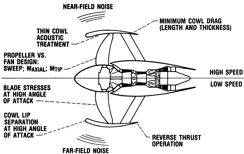
FIGURE 38. - HIGH-SPEED DUCTED PROPELLER ISSUES.
