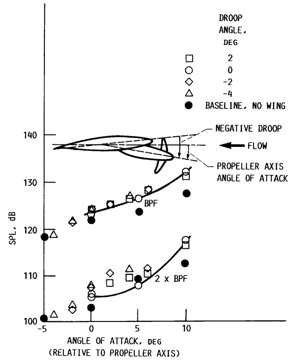
FIGURE 14. - EFFECT OF PROPELLER DROOP ON MAXIMUM TONE NOISE. STRAIGHT WING, 0.54 CHORD SPACING, U_t = 244 M/SEC (800 FT/SEC), \beta = 37.8^\circ , M = 0.2 .
