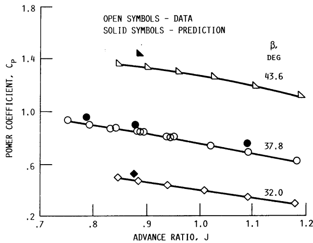
FIGURE 15. - COMPUTED AND MEASURED POWER COEFFICIENTS, M_0 = 0.2 .
