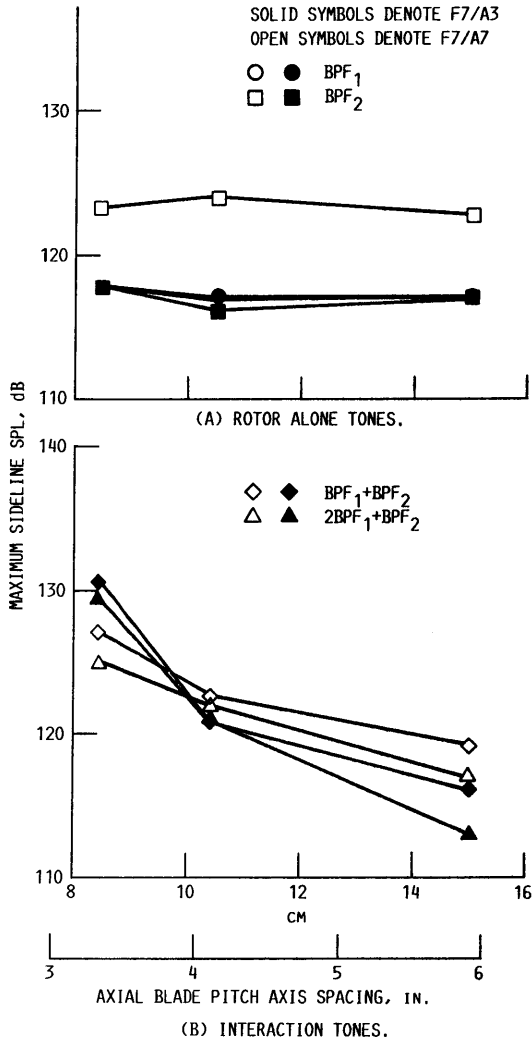
FIGURE 35. - COMPARISON OF F7/A3 AND F7/A7 BLADE ROW SPACING EFFECTS. (137-CM (54-IN.) SIDELINE, 90 PERCENT SPEED, F7/A3, B_1/B_2 = 36.4^0/43.5^0 , F7/A7, B_1/B_2 = 36.4^0/36.5^0 , \alpha = 0^0 , M_\infty = 0.2 .)
