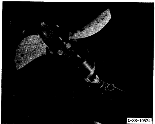
FIGURE 17. - TWO-BLADE VERSION OF LARGE-SCALE ADVANCED PROPFAN (LAP).
