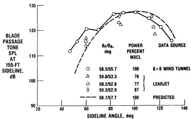
FIGURE 27. - UDF FUNDAMENTAL TONE DIRECTIVITY MEASURED IN FLIGHT, COMPARED WITH SCALED MODEL DATA AND PREDICTION; F7/A7 BLADE CONFIGURATION AT MACH 0.72 CRUISE CONDITIONS.
