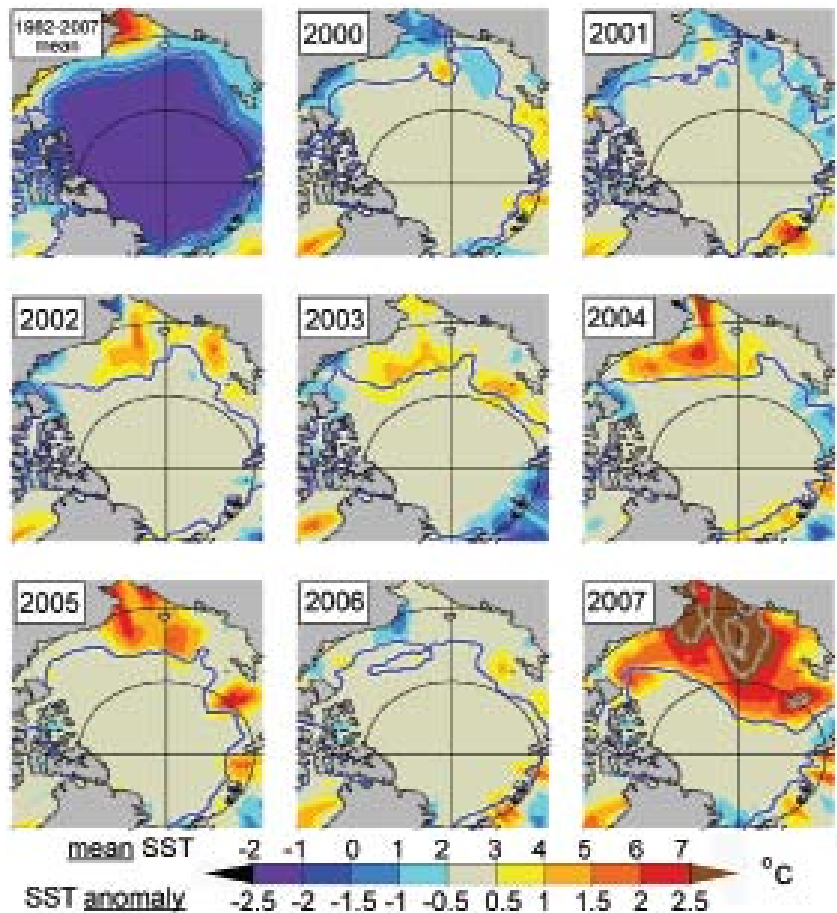
FIG. 5.6. (top left) Mean satellite-derived summer (Jul–Aug) SST (Reynolds et al. 2002) and anomalies from this mean over 2000–07. Latitudes 70^\circ and 80^\circ\text{N} and longitudes 0^\circ/180^\circ and 90^\circ\text{E}/270^\circ\text{E} are shown. For 2007, extra contours for 3^\circ and 4^\circ\text{C} are provided. Also shown is the Sep mean ice edge (blue contour) for each year (from Steele et al. 2008).
