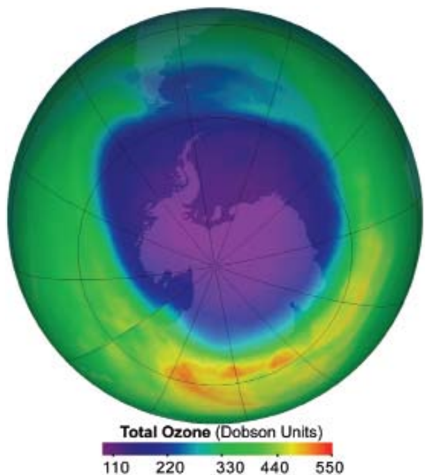
FIG. 5.27. Total ozone (in DU) measured on 30 Sep 2007. Purple blue coloring indicates the low values of the Antarctic ozone hole. The minimum value observed on this day was 106 DU. The image is based on total ozone observations from the OMI aboard the NASA Aura satellite. From Ozone Hole Watch ( http://ozonewatch.gsfc.nasa.gov/ ).
