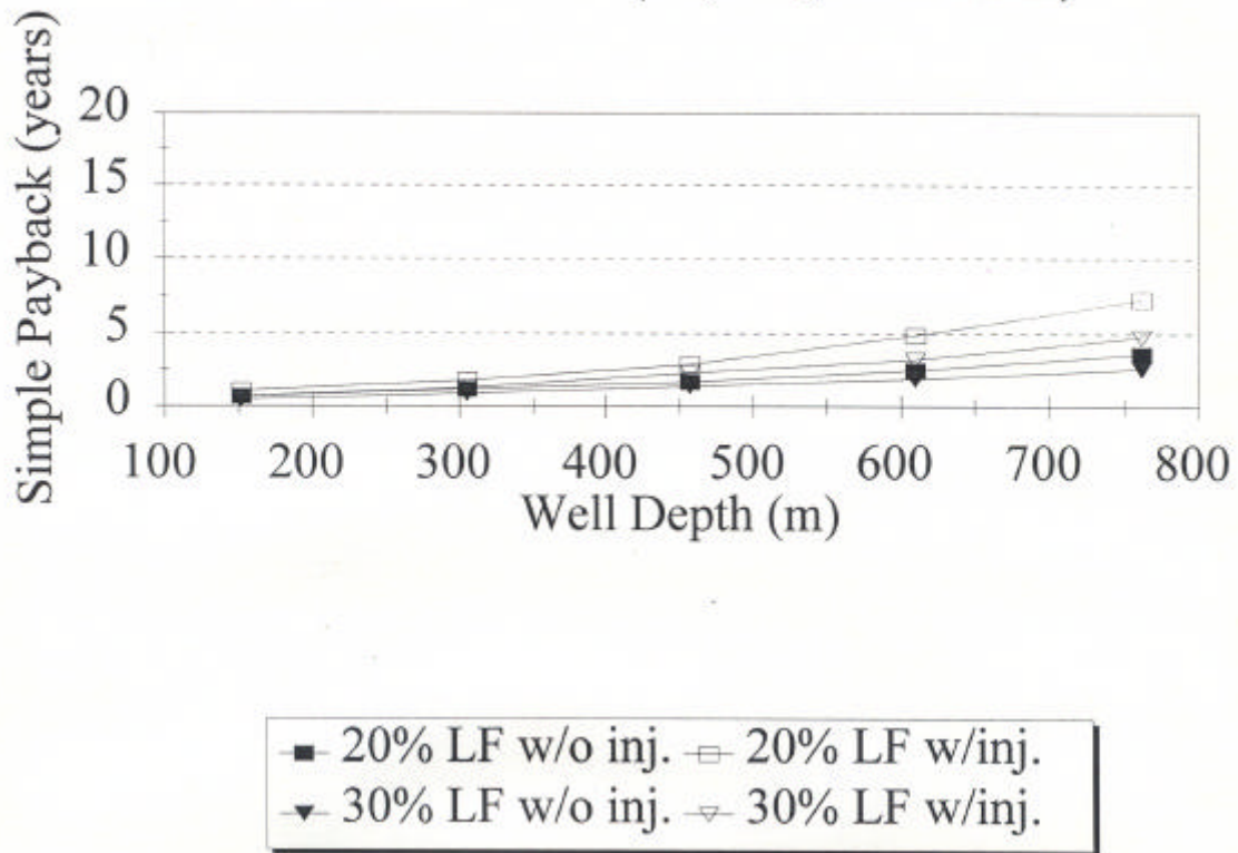
Figure 7. Cost effectiveness of geothermal energy vs. natural gas for a 6 MWt (20,000,000 Btu/hr) load with two production wells.
