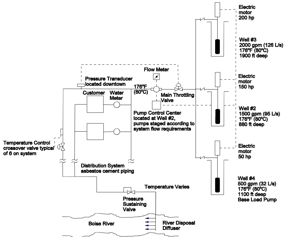
Figure 3. Geothermal district heating system - open distribution.
