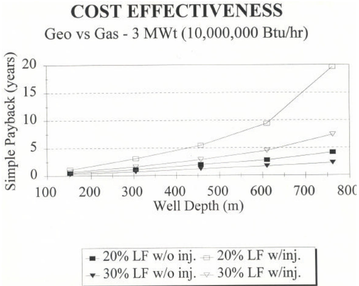
Figure 6. Cost effectiveness of geothermal energy vs. natural gas for a 3MWt (10,000,000 Btu/hr) load with one production well.
