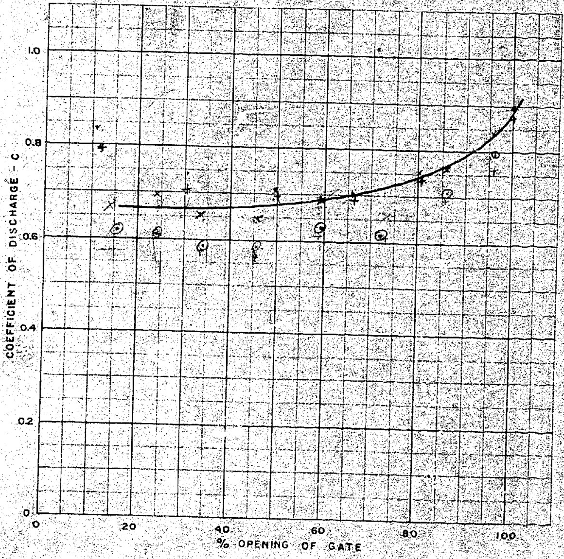
DAVIS DAM RADIAL GATE STUDY COEFFICIENT OF DISCHARGE CURVE
