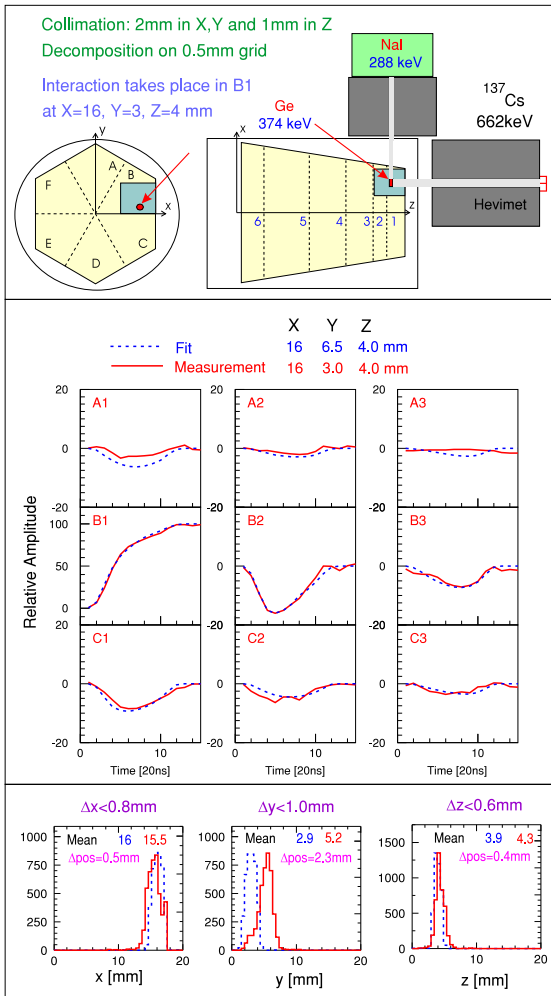
Fig. 2. Top: Coincidence setup used to determine position resolution. Middle: Example of fitted (e.g. calculated) and measured signals. (full lines: measured, dashed lines: fitted) Bottom: Measured (full lines) and simulated (dashed lines) x, y, z positions of interactions.
