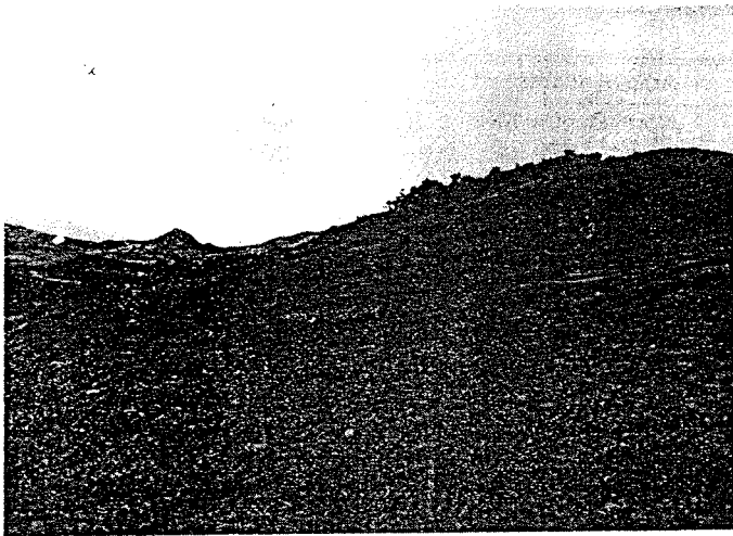
Fig. 3. A rocky hillside northeast of Rosemont with a sparse covering of grass in 1933 (U.S. Forest Service).
