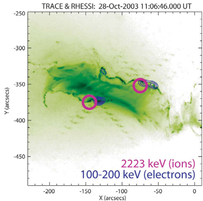
Fig. 5. Imaging of the 2.2 MeV neutron capture line and HXR electron bremsstrahlung emission of the October 28, 2003 flare. The event averaged 2.2 MeV centroid positions (pink circles) and the 100-200 keV contours are superposed on a TRACE EUV 195A image. Both emissions are related to the flares ribbons seen in EUV, but are slightly ( \sim 15'' ) shifted relative to each other. Thermal X-ray emissions of this flare are shown in Fig. 1.
