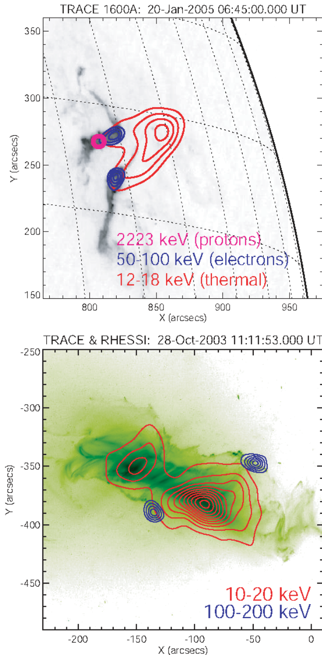
Fig. 1. Solar flare imaging in X-rays of two large X-class two ribbon flares: Thermal and non-thermal X-ray emissions are shown in red and blue contours, respectively. For the January 20, 2005 flare (top) the flare loop is seen mostly from the side, while for the October 28, 2003 flare that occurred near disk center the flare loops are seen from above (bottom). The underlying image shows TRACE observations outlining the flare ribbons. HXR footpoint emissions are typically seen only from some parts of the EUV ribbons, but not along the entire ribbons. The pink circle marks the flare averaged location of the 2.2 MeV line emission in the January 20 flare.
