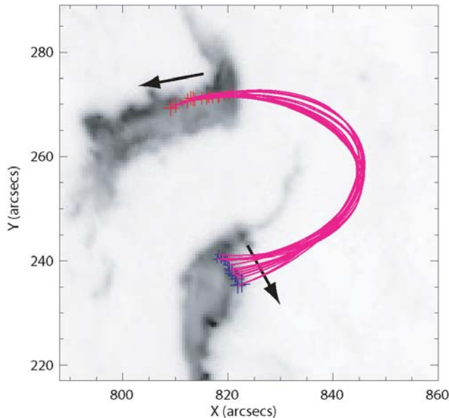
Fig. 2. Temporal evolution of HXR footpoint sources during the January 20, 2005 flare (06:43-06:48 UT). The motion in time of the strongest emission on each flare ribbon is indicated by arrows and increasing symbol size (cadence is of 20 seconds). Simultaneously brightening footpoints are connected by elongated semicircles outlining possible flare loops. The motion of the northern footpoint is clearly along the ribbon, contrary to reconnection models that predict motion perpendicular to the ribbons.
