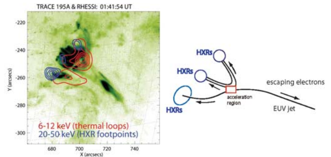
Fig. 4. Solar source region of a flare releasing energetic electrons into interplanetary space that are later observed near Earth: (left) RHESSI X-ray contours at 6-12 keV (red, thermal emission) and 20-50 keV (blue; non-thermal emission) are overlaid on a TRACE 195A-EUV image (dark corresponds to enhanced emission). Around [700,-245], the X-ray emission clearly outlines a loop with two non-thermal footpoints. The strongest non-thermal source however, is slightly to the south east [683,-257] and surprisingly shows a lower intensity thermal source. (Right) Simple magnetic reconnection models (interchange reconnection) predict a similar source structure: The red gray box marks the acceleration site from where downward moving electrons produce the HXR sources and upwards moving electrons escape into interplanetary space. TRACE observation shows a EUV jet outlining the direction of open field lines.
