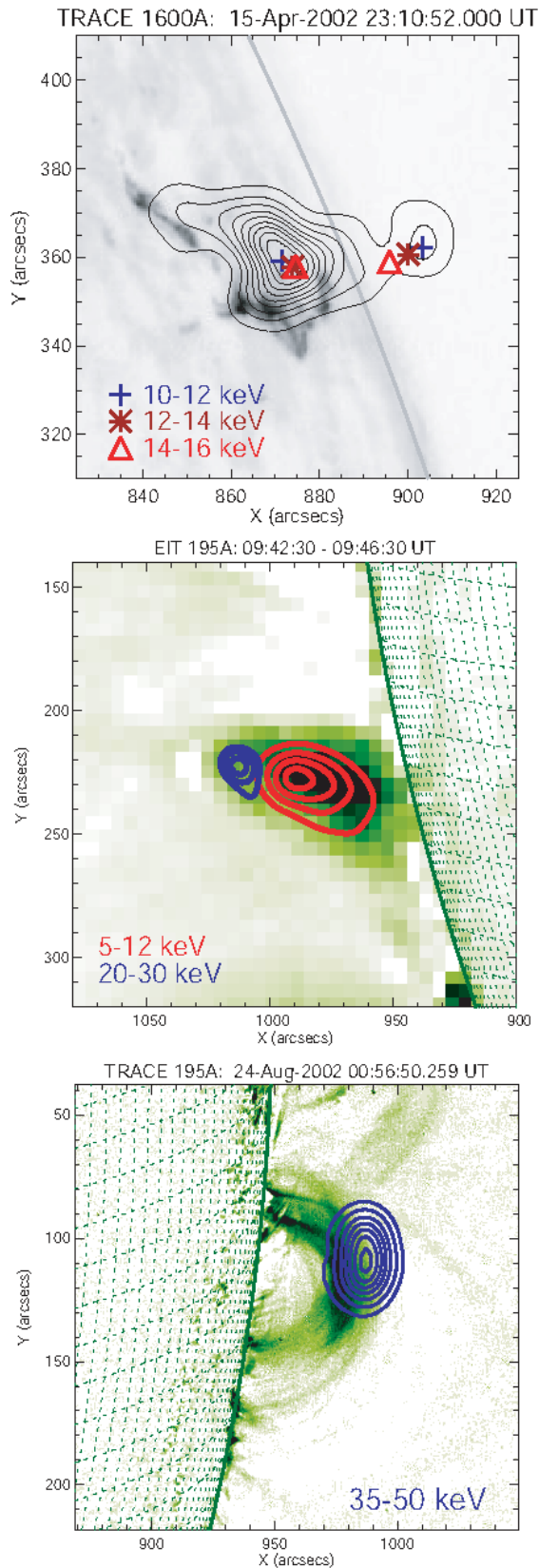
Fig. 3. Example of coronal X-ray emissions from a flare as seen by RHESSI: (top) flare with thermal source above the main flare loop (after Sui & Holman 2003); (middle) HXR ‘above the loop top source’ in a partially occulted flare. The red contours show the thermal flare emission, the blue contours give the location of the ALT source. HXR footpoints are occulted by the solar limb and therefore not visible. (bottom) Coronal hard x-ray source seen before the impulsive phase of an X-class large flare.
