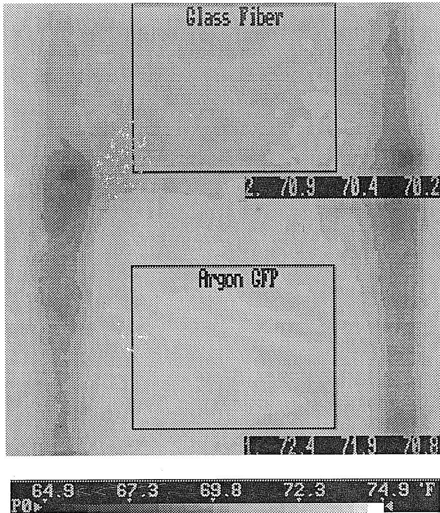
Figure 3. Infrared image of the warm-side surface of a stud wall cavity test section. The upper portion of the cavity is insulated with R-11 h-ft 2 ·°F/Btu (1.9 m 2 ·K/W) glass fiber insulation and the lower portion with a prototype argon GFP. The wall section is constructed with 0.75-in. (0.019-m) plywood, 0.625-in. (0.016 m) drywall and standard 16-in. (0.41-m) on center 2 x 4 studs. The back of this assembly faces a cold chamber at -19.9°F (-28.8°C); ambient temperature is 74.0°F (23.3°C). The warm side surface temperature of the glass-fiber-insulated section averages 70.4°F (21.4°C), while the argon-GFP-insulated section averages 71.9°F (22.1°C). A corresponding temperature gray scale is shown at the bottom of the figure. Since surface temperatures correspond to heat loss rates, the argon GFP's higher warm-side temperature implies a lower heat loss rate.
