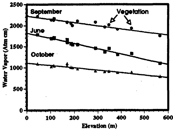
Figure 2. Comparison between atmospheric water vapor and elevation for all of the study sites over the three dates. Water vapor was negatively correlated with elevation (June: Y = -1.236 \cdot X + 1820 , R^2 = 0.966 ; Sept.: Y = -0.759 \cdot X + 2225 , R^2 = 0.875 ; Oct.: Y = -0.576 \cdot X + 1117 , R^2 = 0.896 ).
