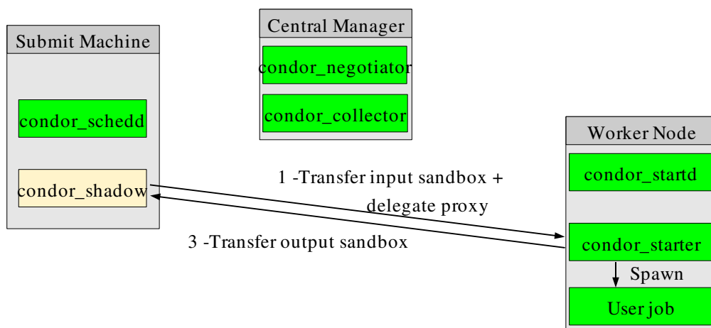
Figure 2.4c: Without identity switching, condor_startd exposed to user attacks
