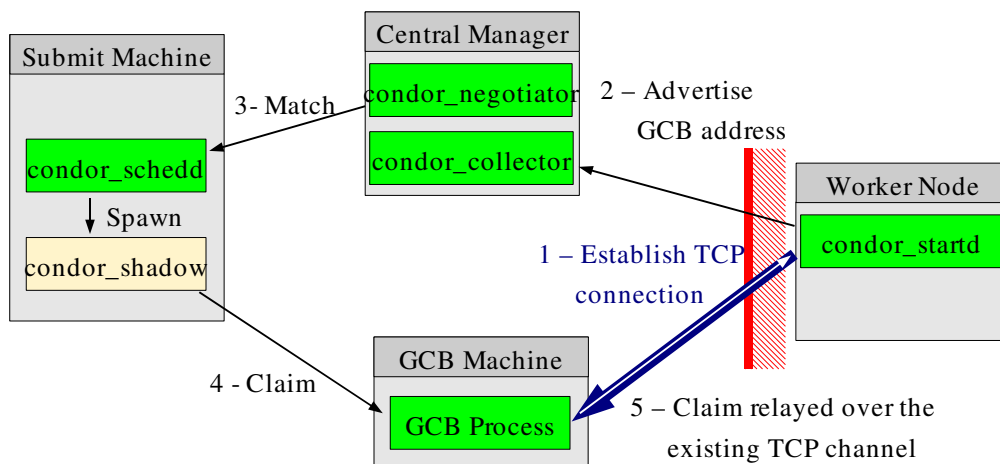
Figure 5: Condor use of GCB to traverse firewalls
