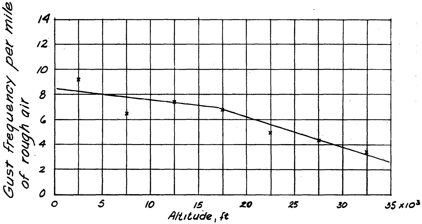
Figure 7.- Gust frequency per mile of rough air as a function of altitude.
