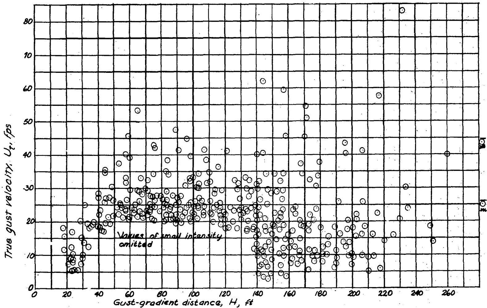
Figure 3.- True gust velocity U_t as a function of the gust-gradient distance H . (Data obtained in 1941 and 1942.)
