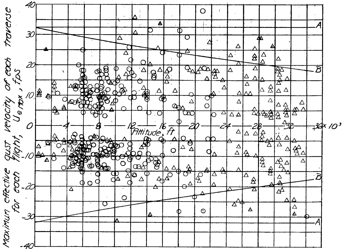
Figure 5.- Maximum effective gust Velocities for each traverse as a function of altitude. (Data obtained in 1941 and 1942.)
