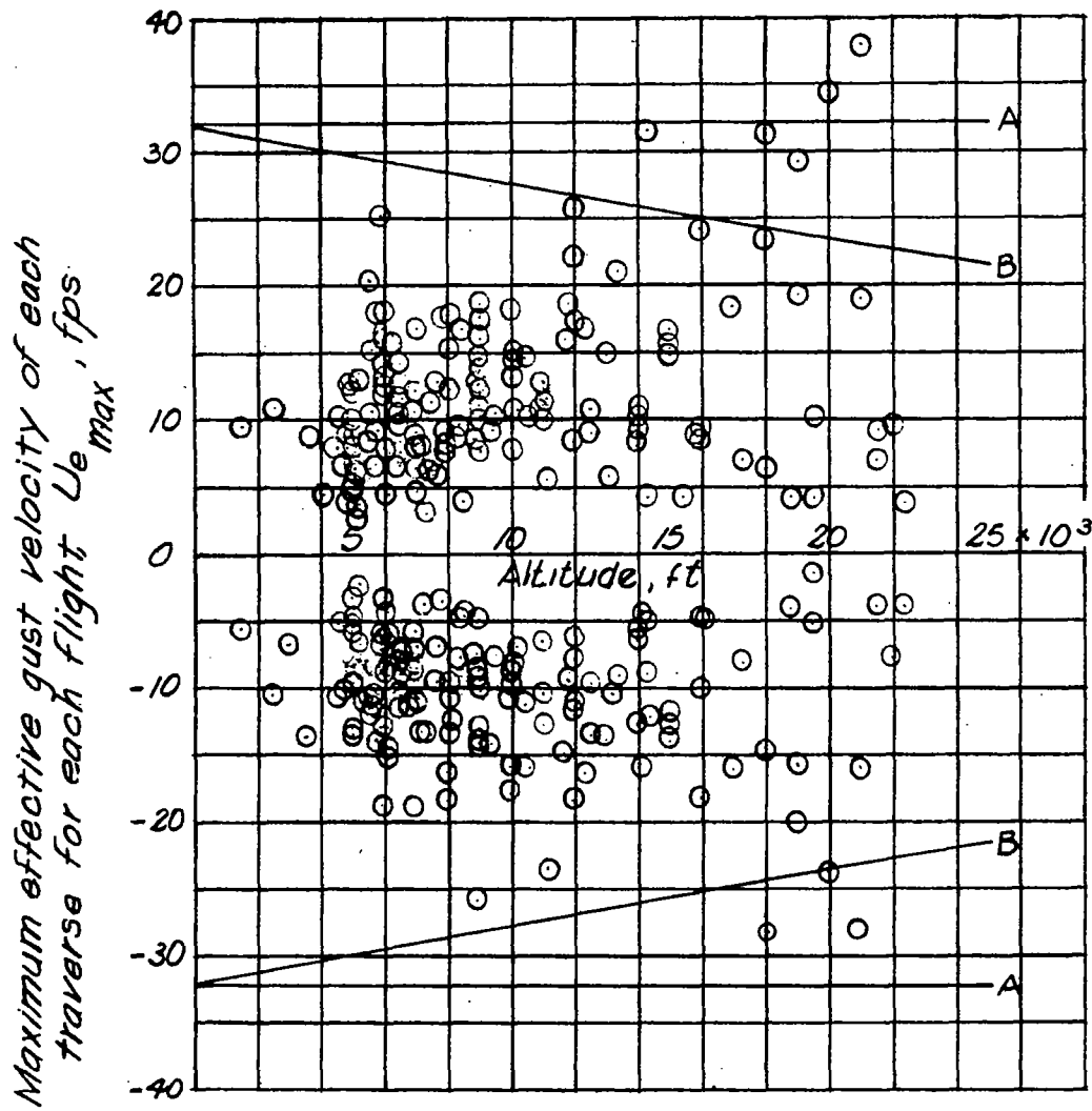
Figure 4.- Maximum effective gust velocities for each traverse as a function of altitude. (Data obtained in 1942)
