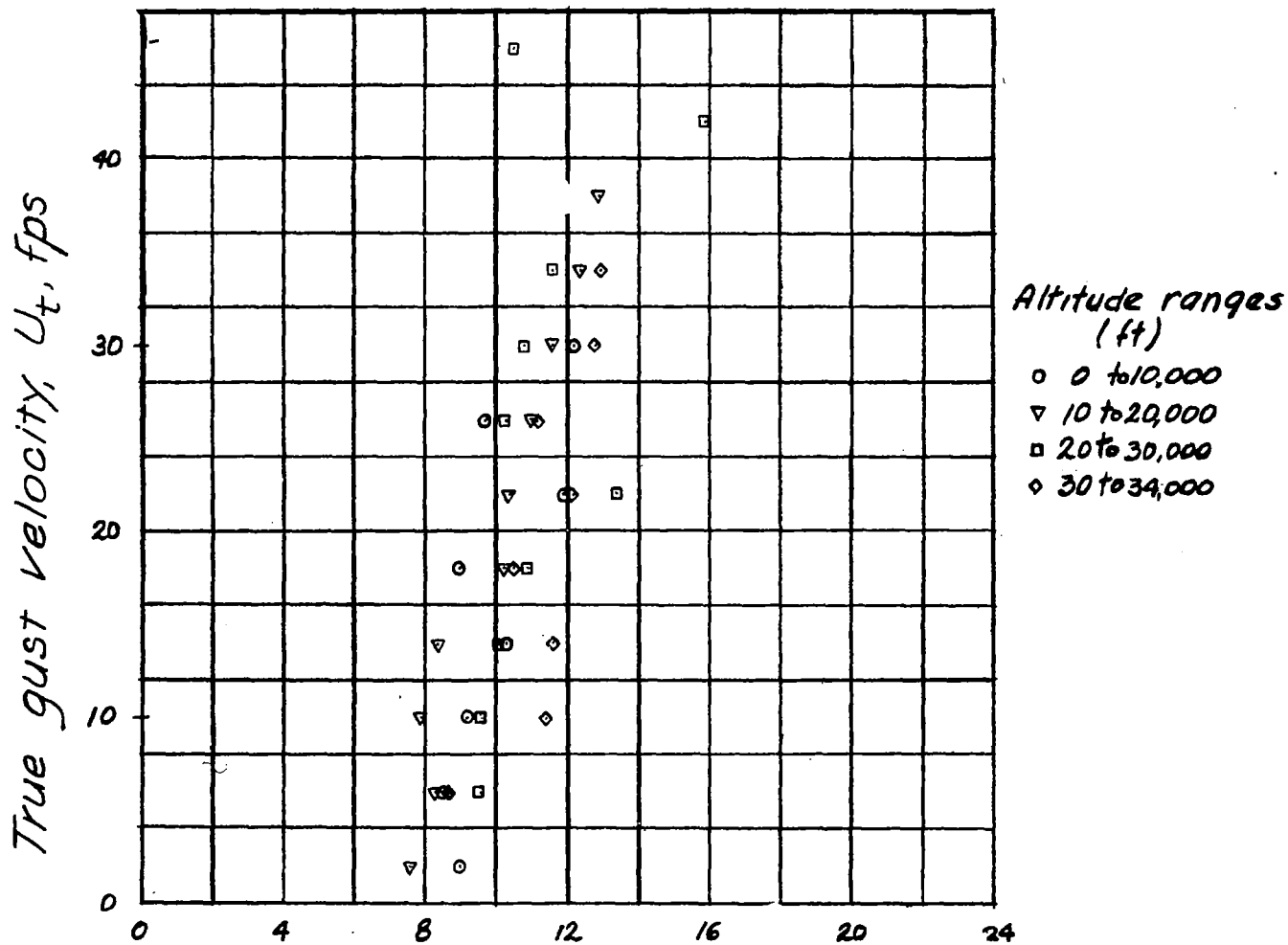
Average gust-gradient distance, H_{av} , chord lengths Figure 6.- Variation of average gust-gradient distance with true gust velocity. (Data obtained in 1941 and 1942)
