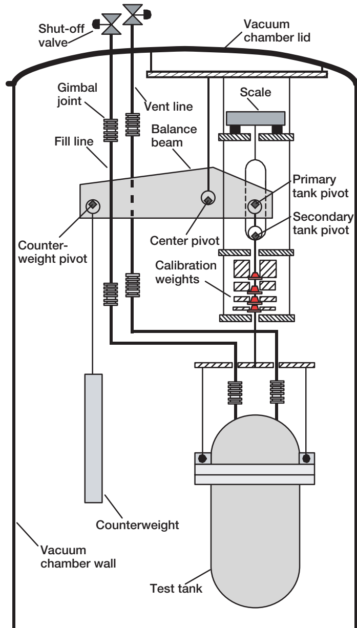
Figure 1.—Schematic of weigh system inside vacuum chamber.
