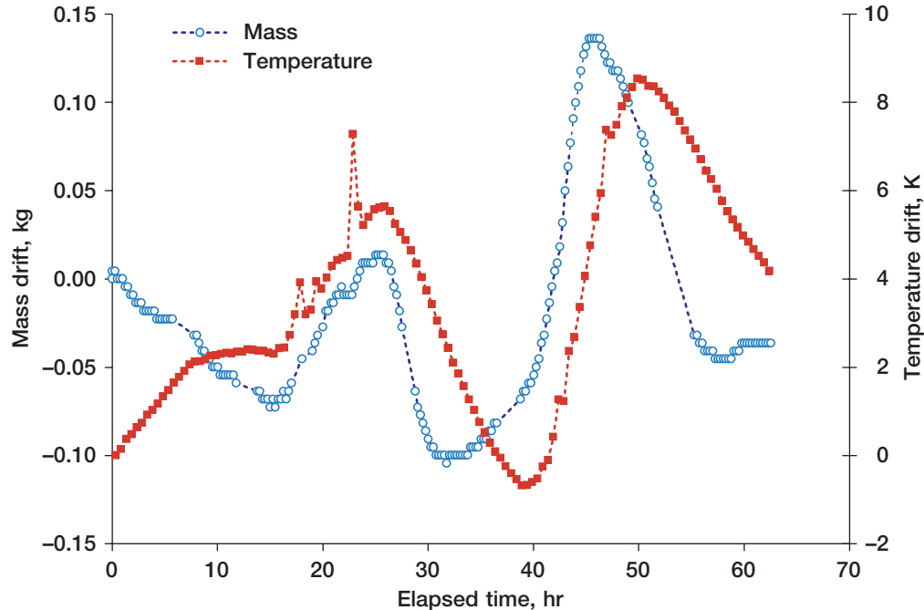
Figure 5.—Long-term drift of scale output and scale temperature excursion.
