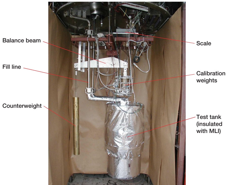
Figure 2.—Photograph of weigh system and insulated test tank outside of vacuum chamber.
