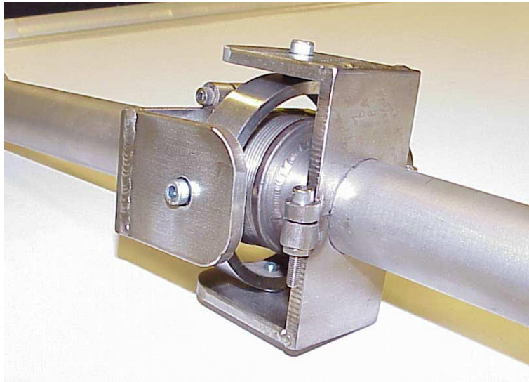
Figure 3.—Photograph of gimbal joint (In final version, yoke-to-tube interface was welded instead of clamped as shown).
