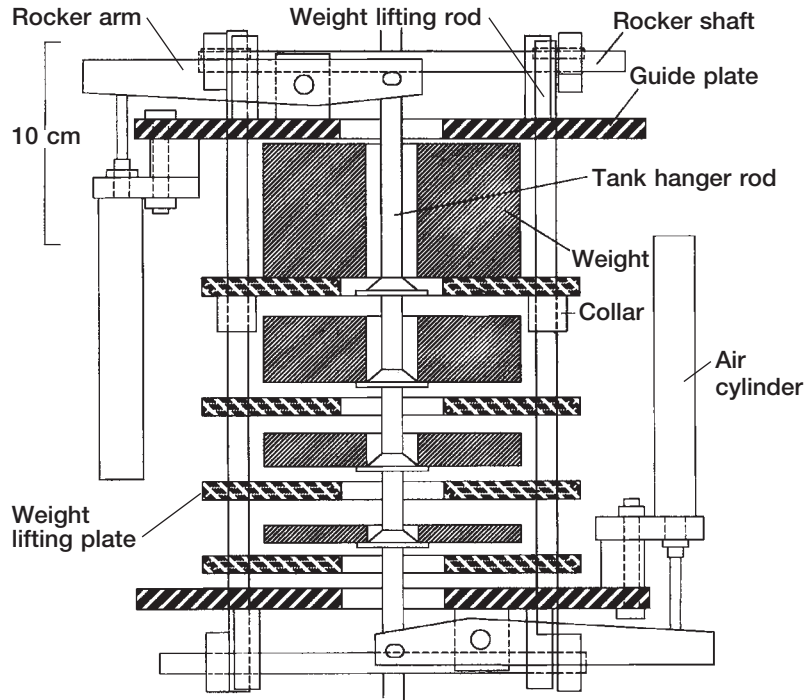
Figure 4.—Schematic drawing of calibration weight sub-assembly.
