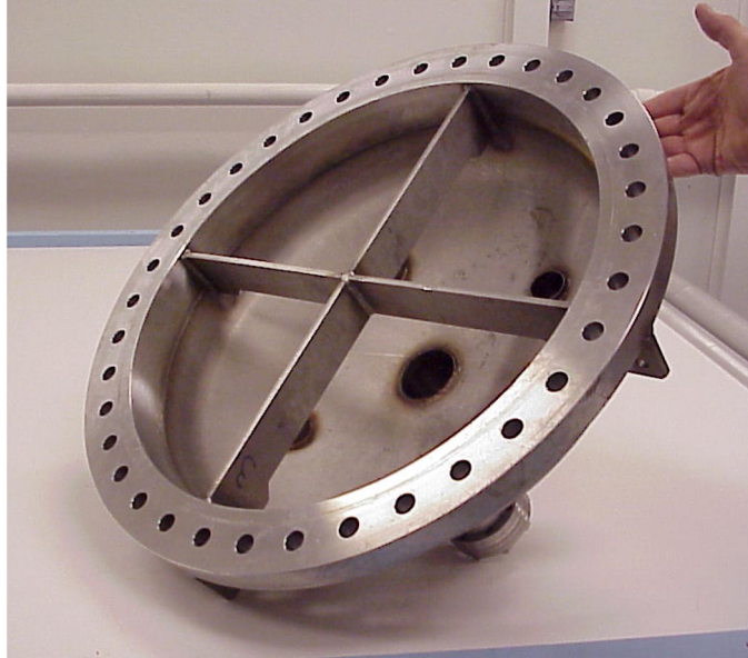
Figure A-3.—Photograph of underside of tank lid showing cross members.
