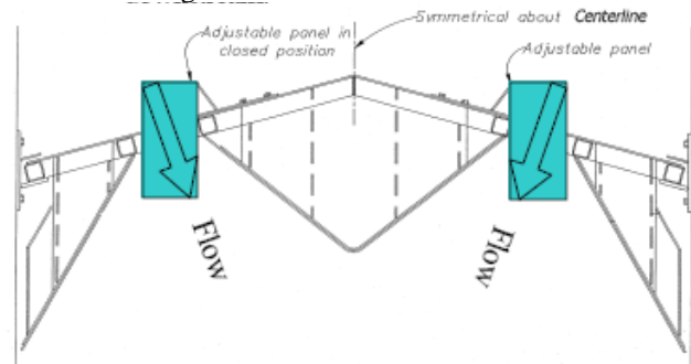
Figure 25 - Horizontal section through dual-vertical slot baffle design.
