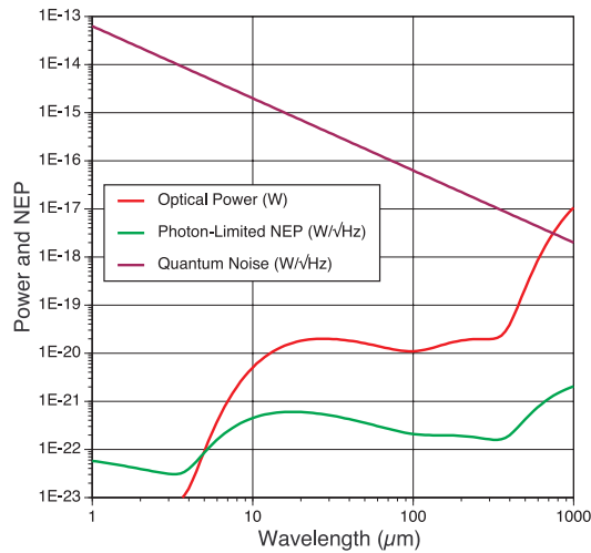
Figure 4. High resolution spectrometer sensitivity.
