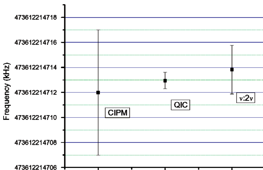
Fig. 4. Comparison between QIC and \nu -to- 2\nu the standard self-referencing technique for optical comb metrology. Both results fall within the uncertainty of the CIPM recommended values. Allan deviations at the best averaging time in our measurements are 0.663 kHz for QIC, and 1.944 kHz for \nu -to- 2\nu .
