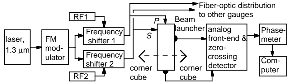
Figure 3: block diagram of metrology system. Building blocks include stable laser source, FM modulator, frequency shifters, fiber-optic distribution system, beam launcher (with attached photodiodes & preamplifiers), corner cube fiducials, analog front-end & zero-crossing detectors, phasemeters, computers & software. The FM modulator linearly sweeps the optical frequency 84 MHz in a triangle pattern for cyclic averaging. The frequency shifters are fed by RF signals 100 kHz apart to create the 100 kHz heterodyne which will be detected by the photodiodes (attached to beam launcher).
