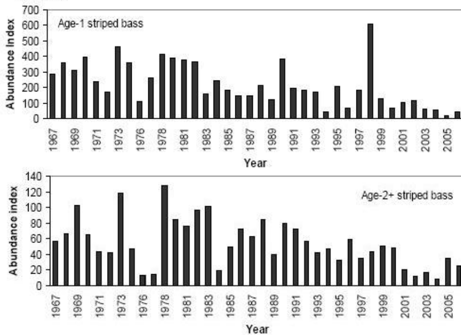
Figure 7-15 Abundance of age-1 and age-2+ striped bass in midwater trawls in A) San Francisco Bay based on the California Department of Fish and Game Bay study (Bay Study) and B) in the Delta from the Fall Midwater Trawl.
