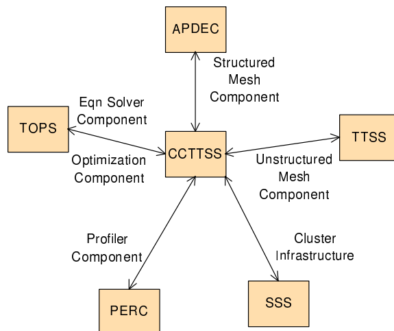
Figure 1.1: Diagram showing the relationship of the CCTSS to other SciDAC ISICs and key interactions.
