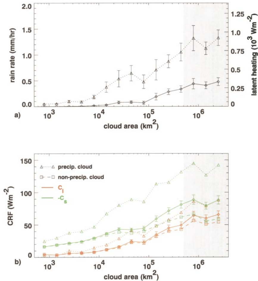
FIG. 5. Cloud-averaged properties as a function of cloud area. (a) Rain rate; right-side axis scaled to show vertically integrated latent heating; (b) C_i (red) and -C_s (green). Solid lines are averages over entire cloud, dotted lines are averages over precipitating portions of cloud, and dashed lines are averages over nonprecipitating portions of cloud. Error bars indicate one standard deviation of the mean.
