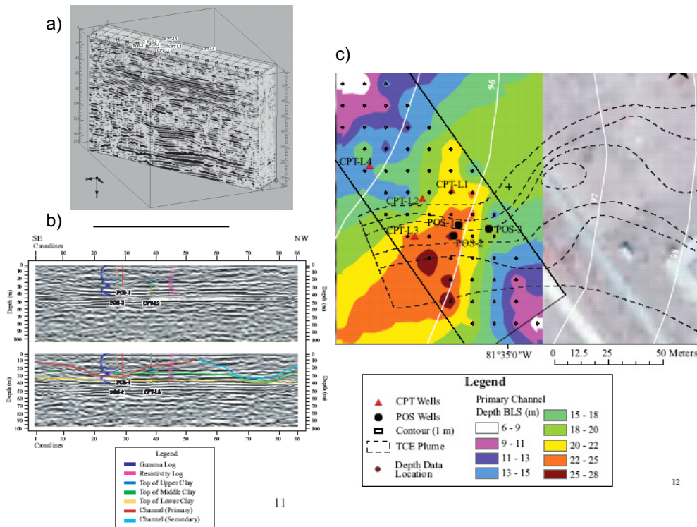
Figure 2. Surface seismic reflection datasets collected at the TCE contaminated Savannah River Site. (a) Pseudo 3D processed seismic data cube. (b) Example of the comparison between geophysical log and seismic reflectors. (c) Comparison of the TCE plume boundary (obtained using wellbore data) with the location of the mapped buried primary channel (obtained using seismic reflection data); the contaminant source is located to the right of the displayed image (modified from Addison et al., 2009).
