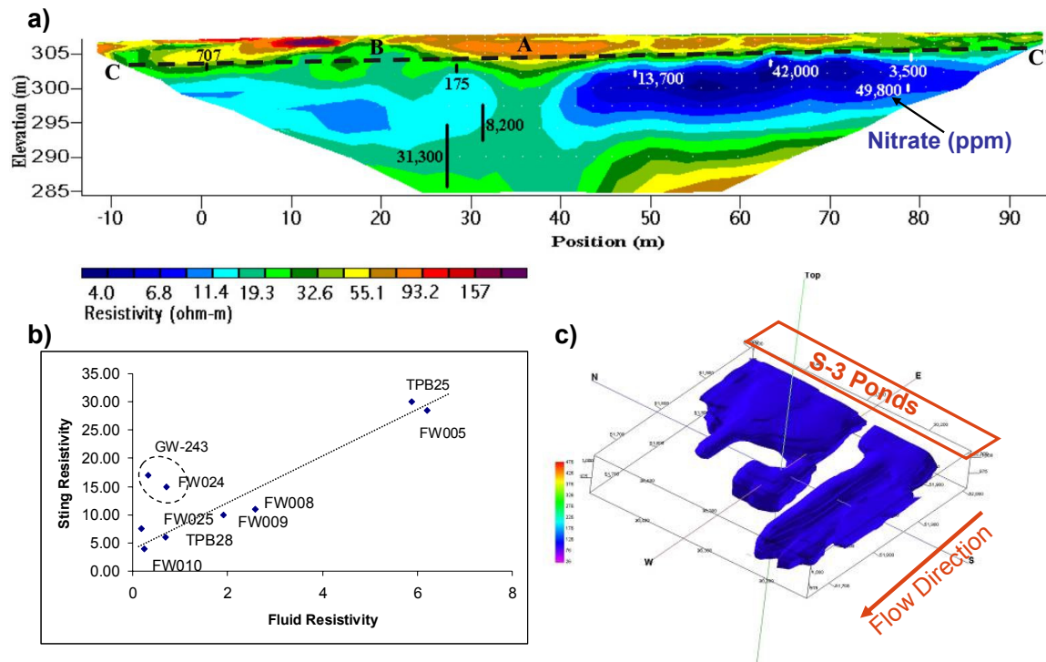
Figure 5. Use of surface electrical datasets at the ORNL IFRC to delineate the approximate plume boundary: (a) example surface electrical profile showing distribution of inverted electrical resistivity as well as nitrate concentrations obtained from wellbore sampling; (b) comparison of electrical resistivity obtained using the surface electrical data collected using a Sting system and the wellbore (fluid) resistivity values; (c) estimation of the distribution of the portion of the nitrate plume having a concentration greater than 3,000 ppm obtained using the surface electrical datasets and a site-specific indicator relationship between electrical resistivity and nitrate concentration (modified from Watson et al., 2005).
