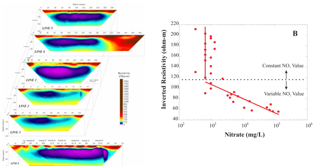
Figure 6. (a) Inverted electrical resistivity profiles at the BC crib area of the contaminated Hanford, Washington Reservation, where the low electrical resistivity (high electrical conductivity) regions were interpreted as the plume boundaries; (b) observed relationship between electrical conductivity and nitrate concentration at a single wellbore location within and above the interpreted plume (modified from Rucker and Fink, 2007).
