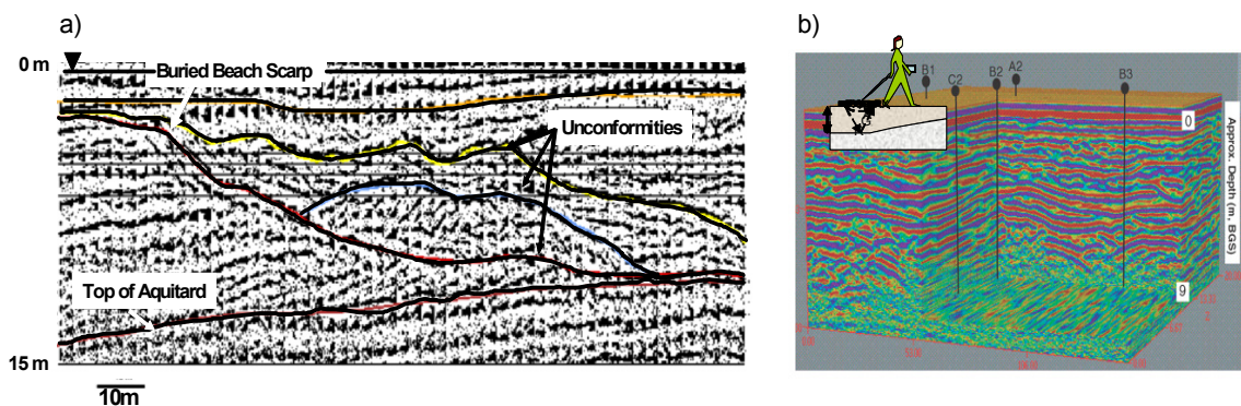
Figure 1. Example of the use of subregional (left) and local scale (right) surface GPR datasets to delineate subsurface stratigraphy at the DOE Oyster Bacterial Transport Site in Oyster, Virginia (modified from Hubbard et al., 2001)
