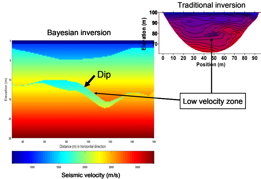
Figure 4. Estimated 2D velocity profile obtained using synthetic seismic refraction data within the developed Bayesian framework with constraints from several boreholes, showing the ability of the estimation framework to more discretely identify the base of the fill, top of the saprolite, and low seismic velocity transition zone at the ORNL IFRC relative to traditional inversion procedures (modified from Chen et al., 2008).
