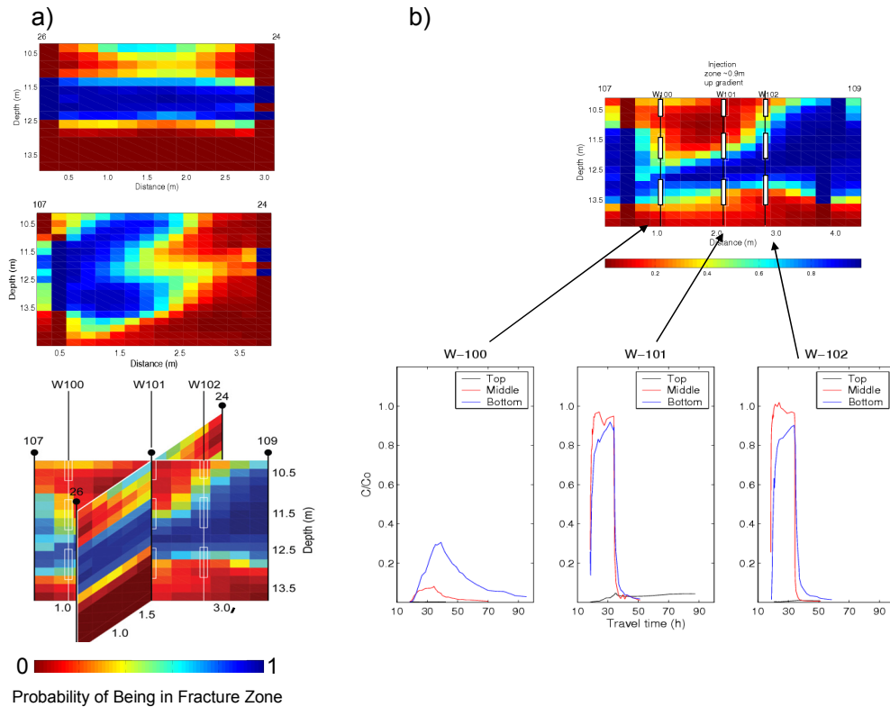
Figure 3. Estimates of natural fracture zonation obtained using seismic tomographic slowness measurements data within a stochastic estimation framework (modified from Chen et al., 2006): (a) estimates along the strike (top) and dip (middle) direction, as well as composite fence diagram (bottom); (b) comparison of the estimated fracture zonation with bromide breakthrough datasets (from Wu et al., 2006) associated with multilevel samplers.
