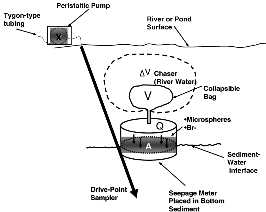
FIG. 3. Schematic of seepage meter illustrating components used in injection and recovery experiments with fluorescently labeled microspheres. Dimensions of seepage meter ( \sim 70 cm wide \times 24 cm high), approximate volume of meter when placed (66 L), drive point sampling wells (15 cm long) were placed at 25 and 50 cm below river or basin sediment surface. Collapsible bag was filled with 1 L of injection mixture and attached to seepage meter; an instantaneous seepage rate could be obtained by noting changes in volume over time.
