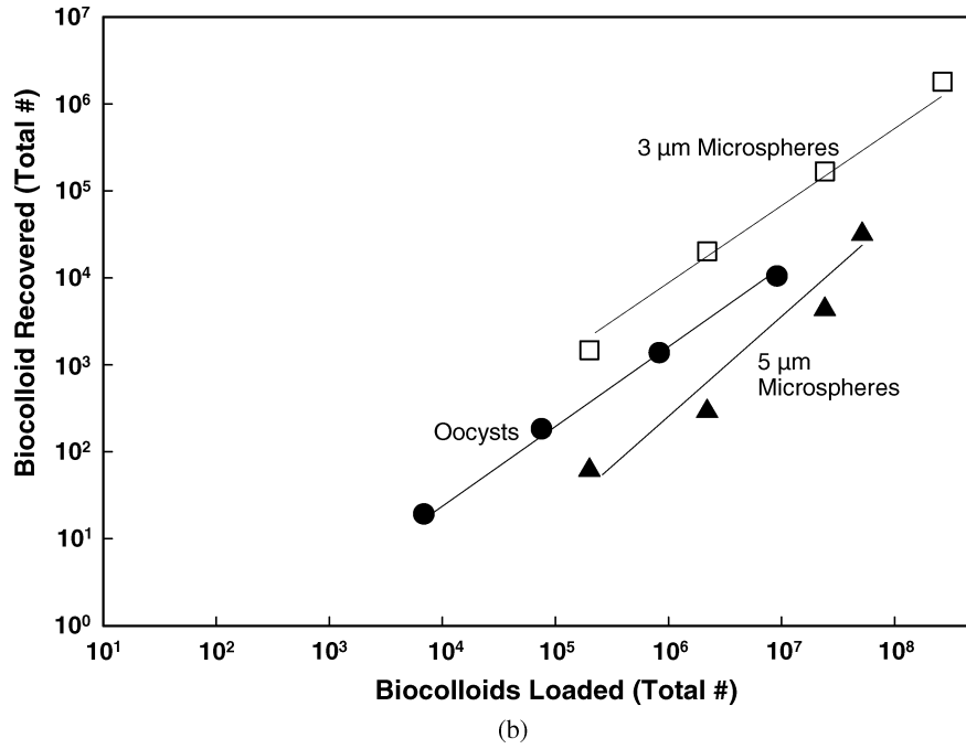
FIG. 6b. Comparison of Cryptosporidium parvum oocysts, 3-µm and 5-µm fluorescent microspheres loaded and desorbed from Russian River infiltration basin sediments. Experiment performed in static minicolumns with 15 grams of sediment at 15°C over a 3-hour incubation time. Concentrations determined using flow cytometry (Biorad HS-Bryte with 103W HBO Hg lamp, and UV FITC excitation filter cube with GR1 and OR1 emission wavelength discrimination cubes and standard forward and side-scatter photomultipliers).
