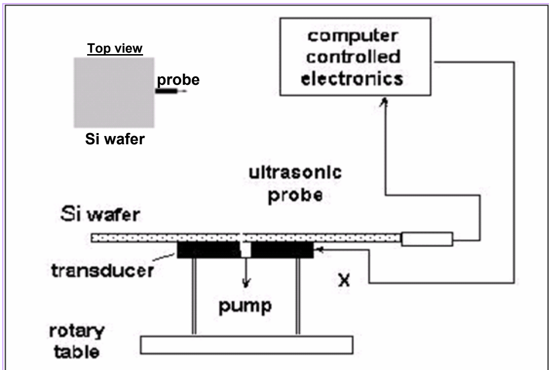
Figure 1. Ultrasonic crack detection apparatus schematic. [Courtesy of the University of South Florida (USF)].
