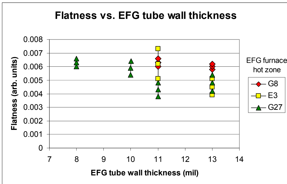
Figure 8. Plot of flatness metric as a function of tube wall thickness. A level of approximately 0.002 corresponds to a flatness yield of > 98%. All runs are for a 12.5 cm EFG furnace.
