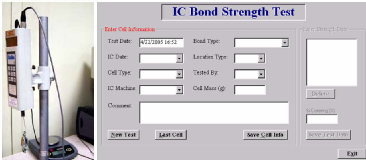
Figure 15. Apparatus and operator interface for data collection of bond strengths for cells in Module Fabrication area tested as for interconnection (IC) quality control.
