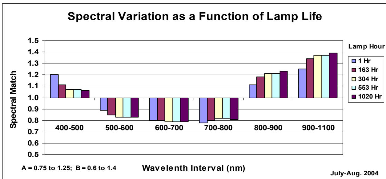
Figure 4. Spectral aging for solar simulator lamp in new cell line as determined using a spectroradiometer.
