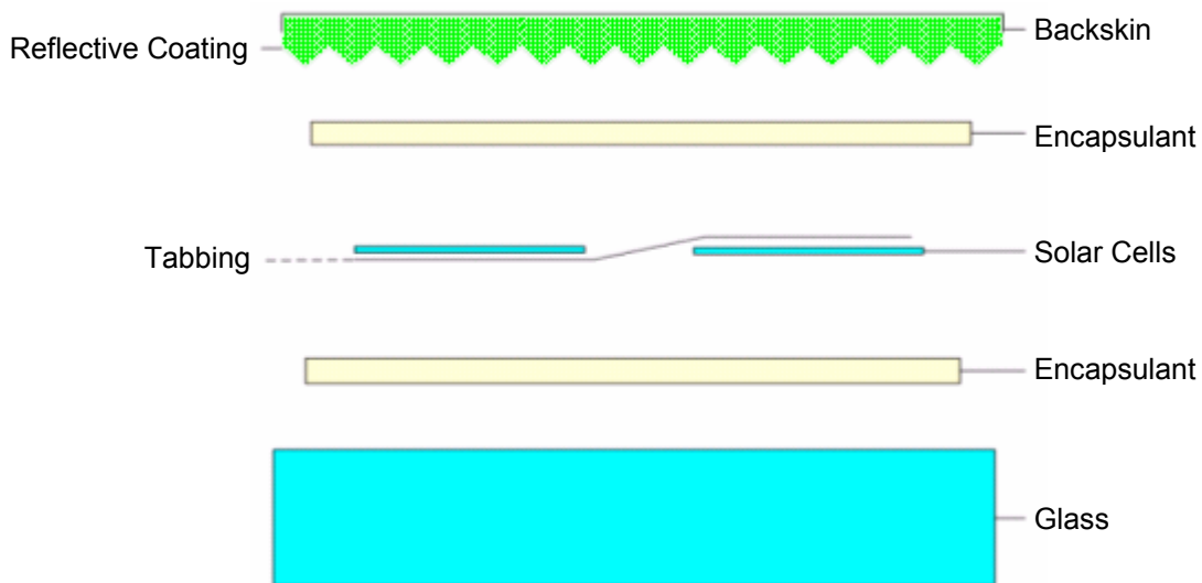
Figure 10. Schematic of reflector module laminate layout.
