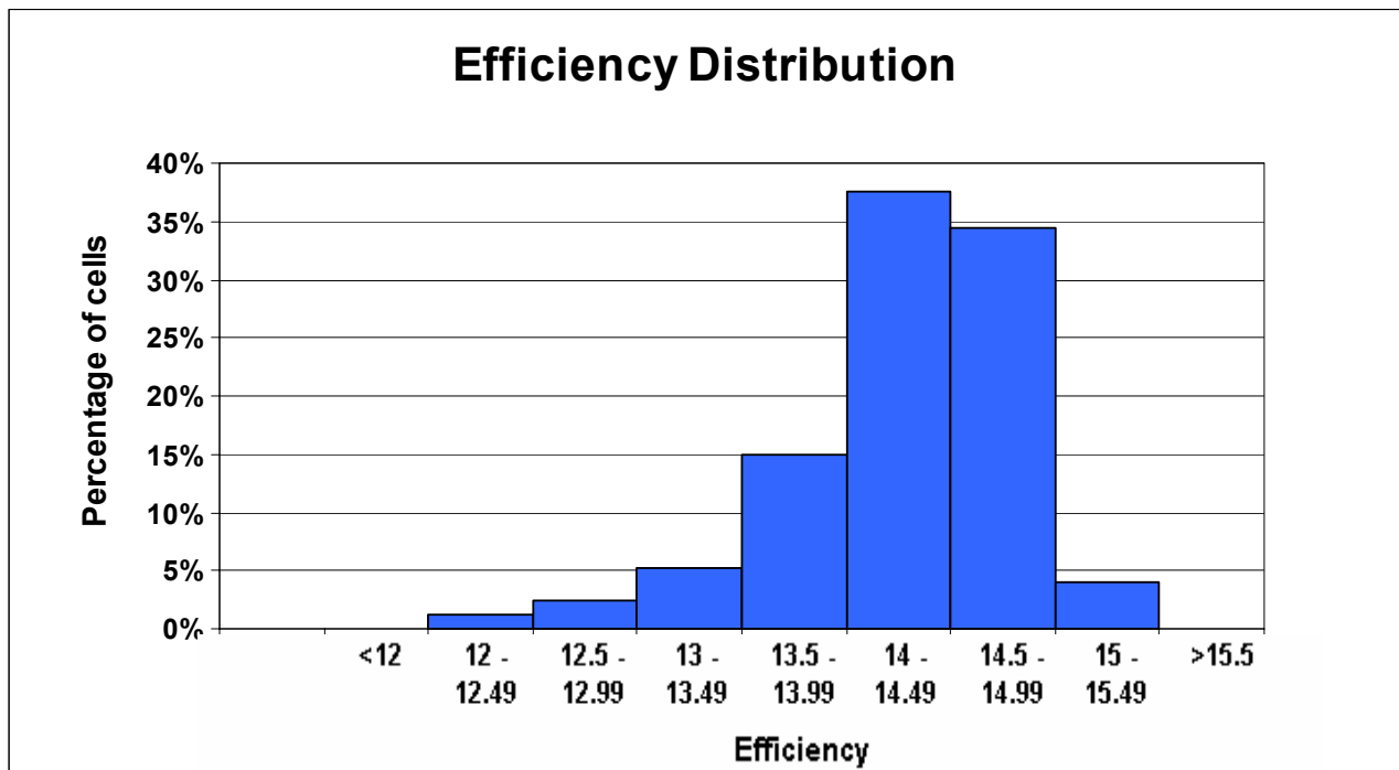
Figure 16. Cell efficiency distribution for 13,000 production cells averaging 14.3%.
