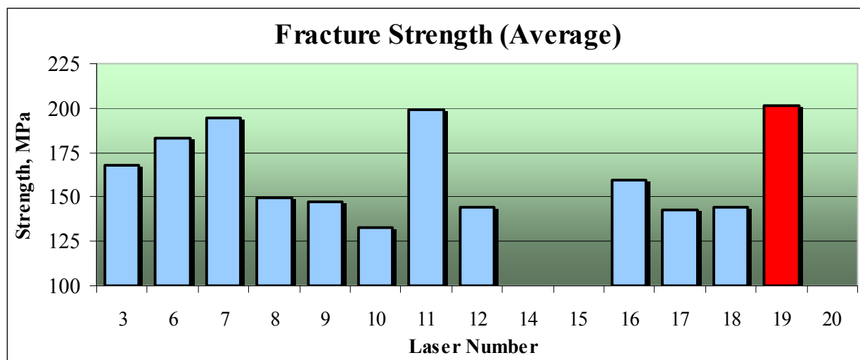
Figure 19. Fracture Strength of EFG silicon wafers cut on different laser cutting stations. Laser 19 represents a new cutting technology being substituted for older lasers.
