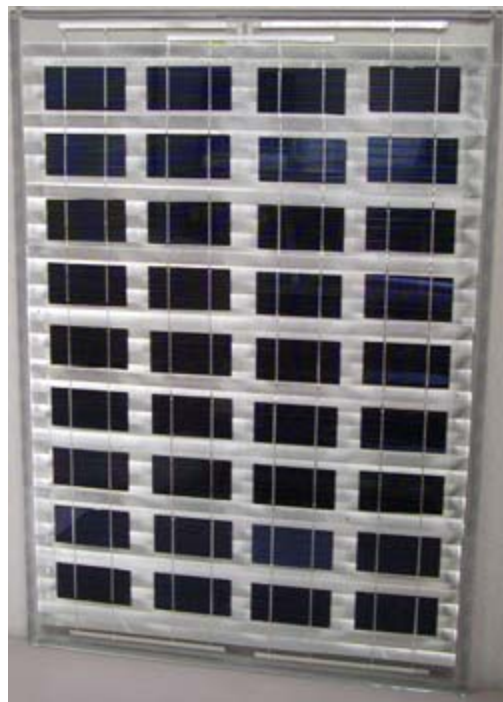
Figure 9. Reflector module incorporating thirty-six 5 cm x 10 cm EFG cells.
