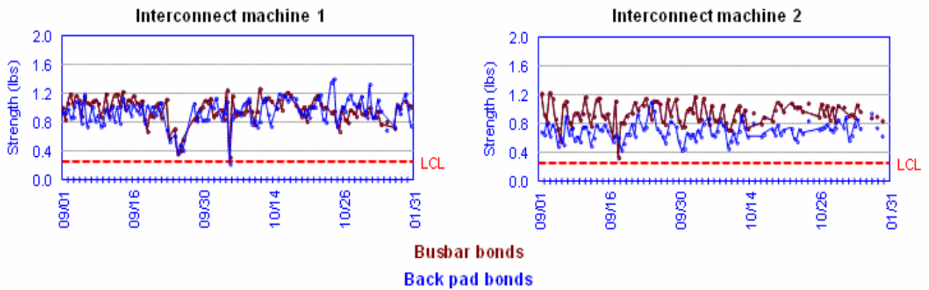
Figure 6. Bond strength SPC charts for two interconnect machines in module manufacturing.
