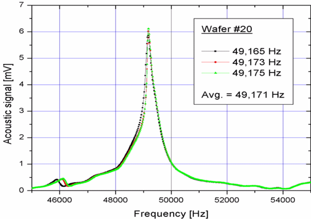
Figure 2. Multiple scans of a silicon wafer by ultrasonic crack detection apparatus showing excellent reproducibility. [Courtesy of the University of South Florida].
