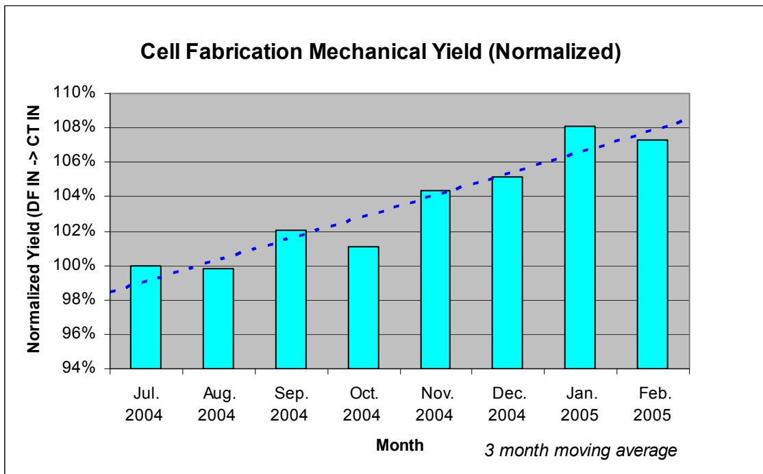
Figure 18. Cell fabrication yield improvements in Phase 3 of this program.
