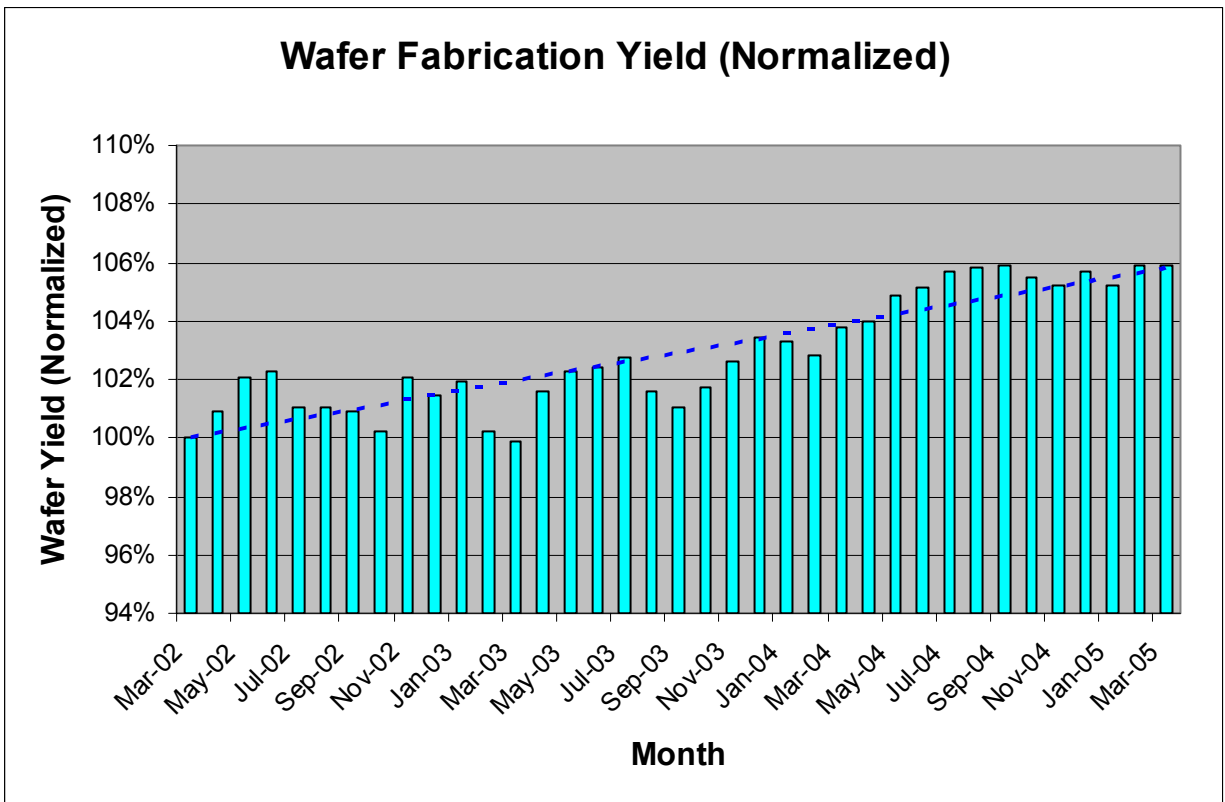
Figure 17. Wafer fabrication yield improvements over the 3 years of this program.
