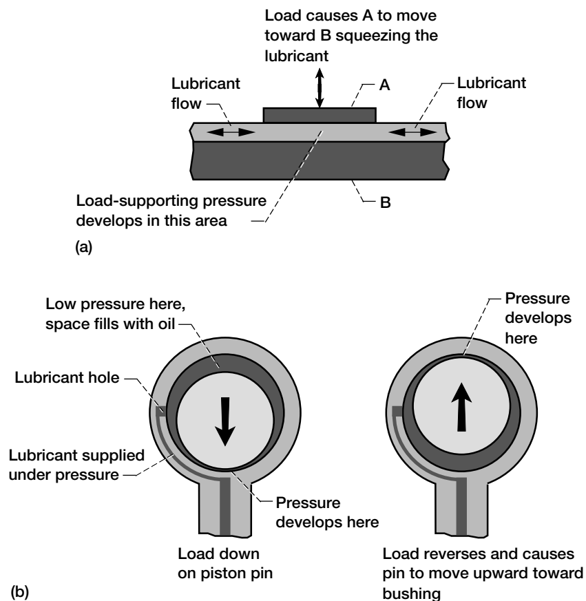
Figure 1.7.—Squeeze film bearing. (a) Squeeze film principle. (b) Squeeze film in piston pin bushing.
