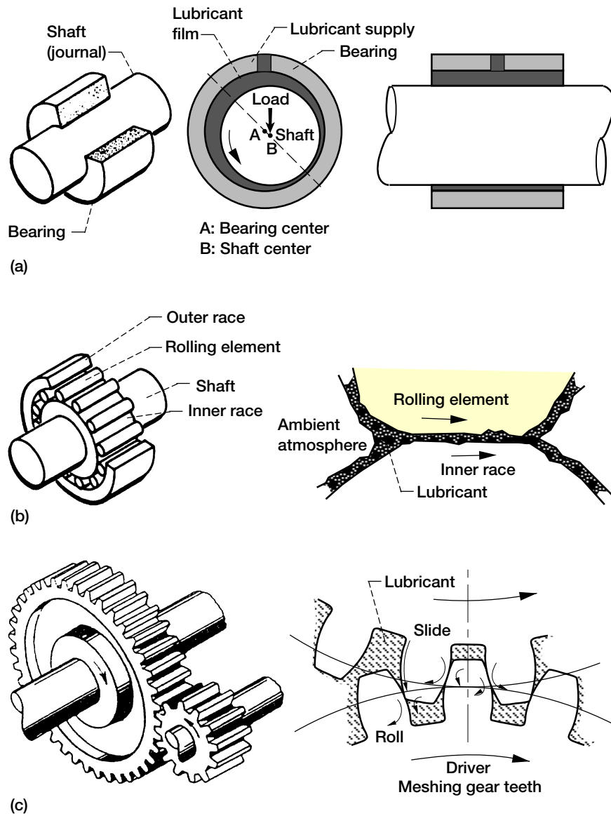
Figure 1.2.—Plain bearings, rolling-element bearings, and gears. (a) Plain bearings based on sliding action. (b) Rolling-element bearings based on rolling action. (c) Gears based on rolling and sliding action.
