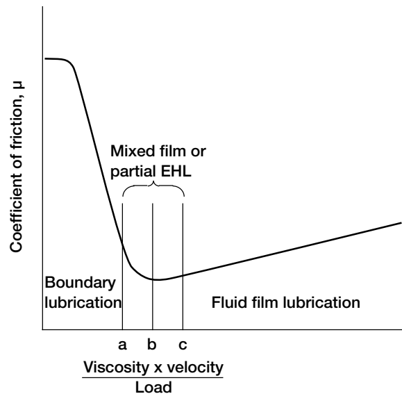
Figure 1.8.—Variation in coefficient of friction with viscosity, velocity, and load for fluid-lubricated sliding bearing (the Stribeck curve).
