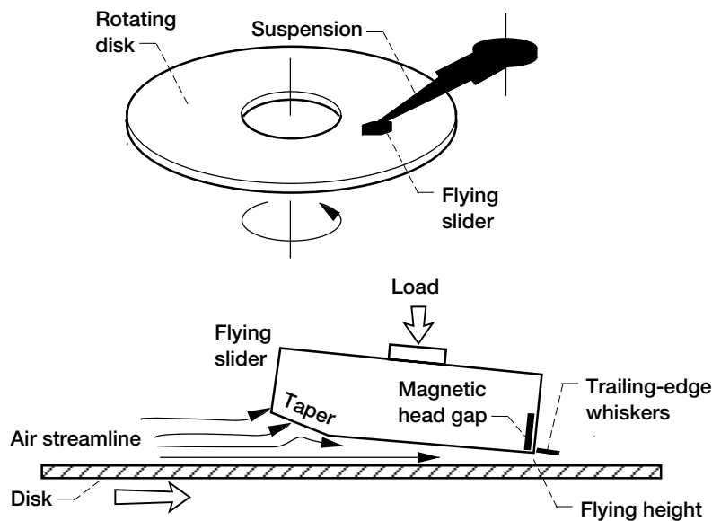
Figure 1.5.—Hydrodynamic gas (air) film lubrication in magnetic hard-disk drive system.
