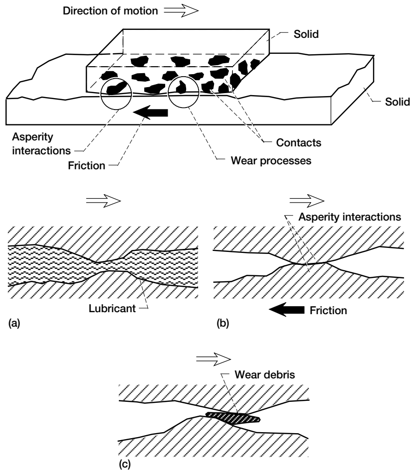
Figure 1.1.—Definition of tribology. (a) Lubrication. (b) Adhesive bonding. (c) Wear.
