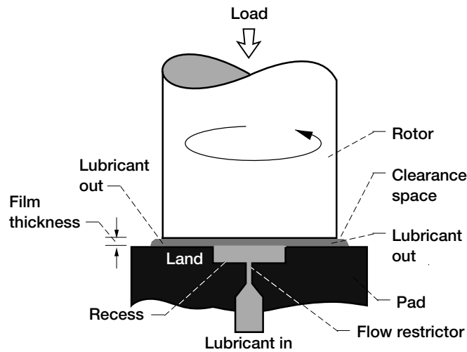
Figure 1.6.—Simple hydrostatic thrust bearing.
