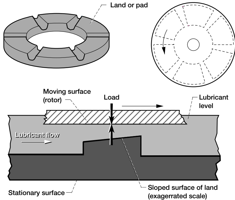
Figure 1.4.—Tilting-pad or tapered-land thrust bearing.
