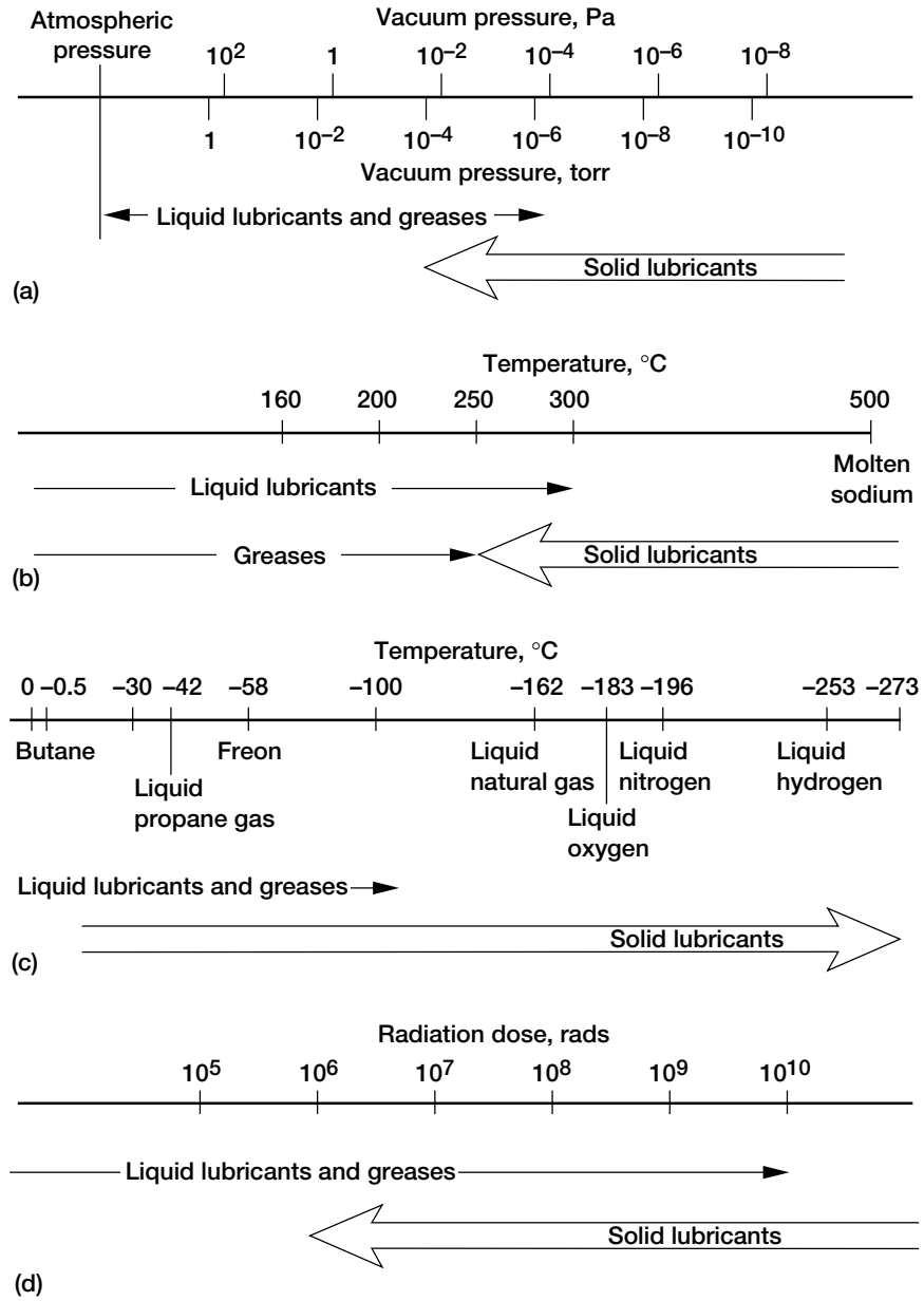
Figure 1.3.—Ranges of application of solid lubricants in (a) high vacuum, (b) high temperature, (c) cryogenic temperature, and (d) radiation environments.
