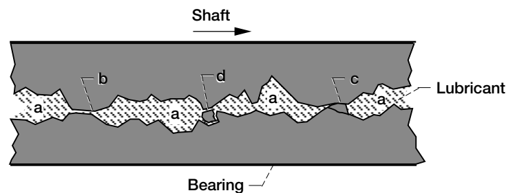
Figure 1.9.—Actions involved in boundary lubrication.
