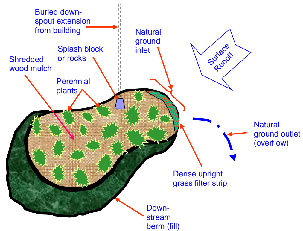
Figure 3. Plan View of Rain Garden
