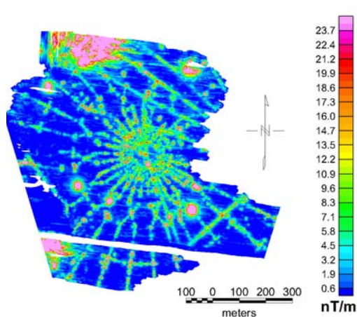
Figure 4. Analytic signal map for a site in Maryland showing anomalies associated with a network of piping that had been overlooked in more localized ground-based surveys.
