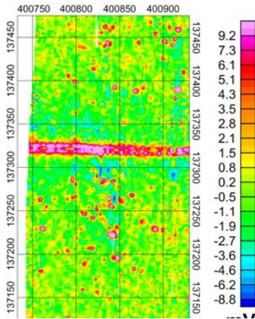
Figure 8. ORAGS-TEM measurements with large loop receiver at a bombing target in South Dakota, corresponding to the magnetic data shown in Figure 6. Data were acquired at 3m flight line spacing. Horizontal scale is in meters.
