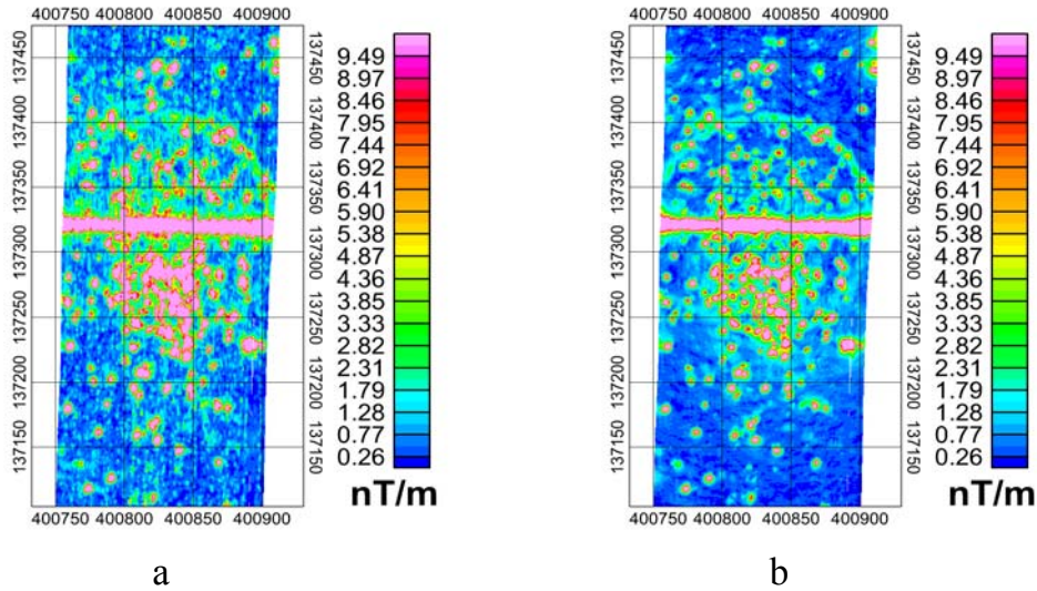
Figure 6. Analytic signal maps for a bombing target in South Dakota. a) Analytic signal derived from total field measurements with the ORAGS-Arrowhead system; b) Analytic signal derived from measured vertical gradient with the ORAGS-VG system. Horizontal scale is in meters.
