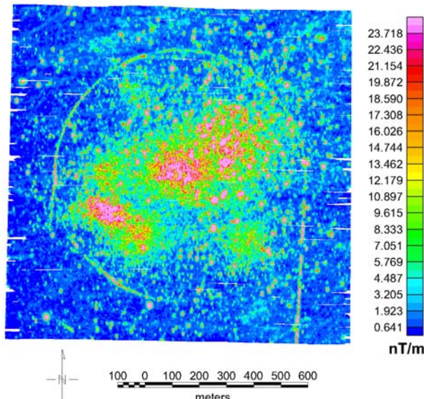
Figure 2. Analytic signal map of a bombing target in New Mexico, derived from airborne magnetic data.
