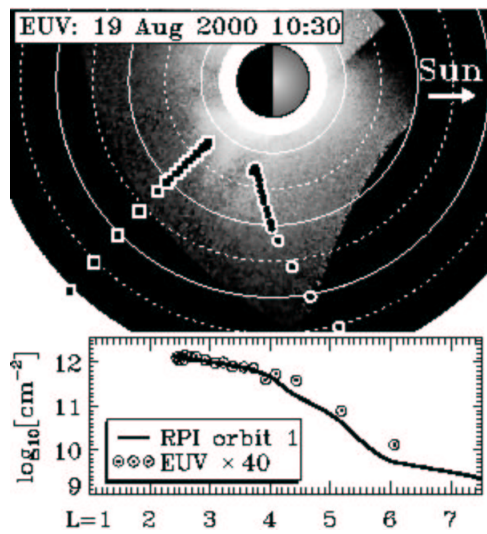
Figure 4. IMAGE EUV intensity at 1030 UT (top panel). IMAGE EUV and RPI column abundances along co-rotated orbit 1 (circles and solid line, respectively) for 1030 UT (bottom panel; see text for details).
