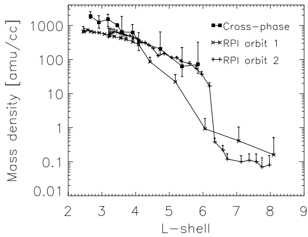
Figure 2. Cross-phase and IMAGE RPI derived plasma mass densities with associated error bars (see text for details).
