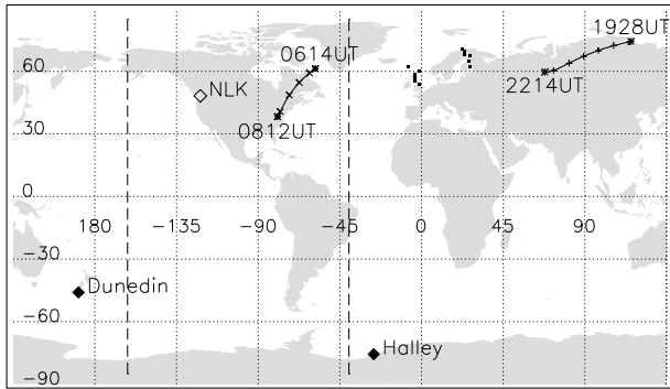
Figure 1. Map showing relative geographic positions of the instruments used for this study. IMAGE satellite northern-hemisphere magnetic field traces between 0614 – 0812 UT and 1928 – 2214 UT are also shown, with tick marks placed at hh:00 and hh:30 UT.
