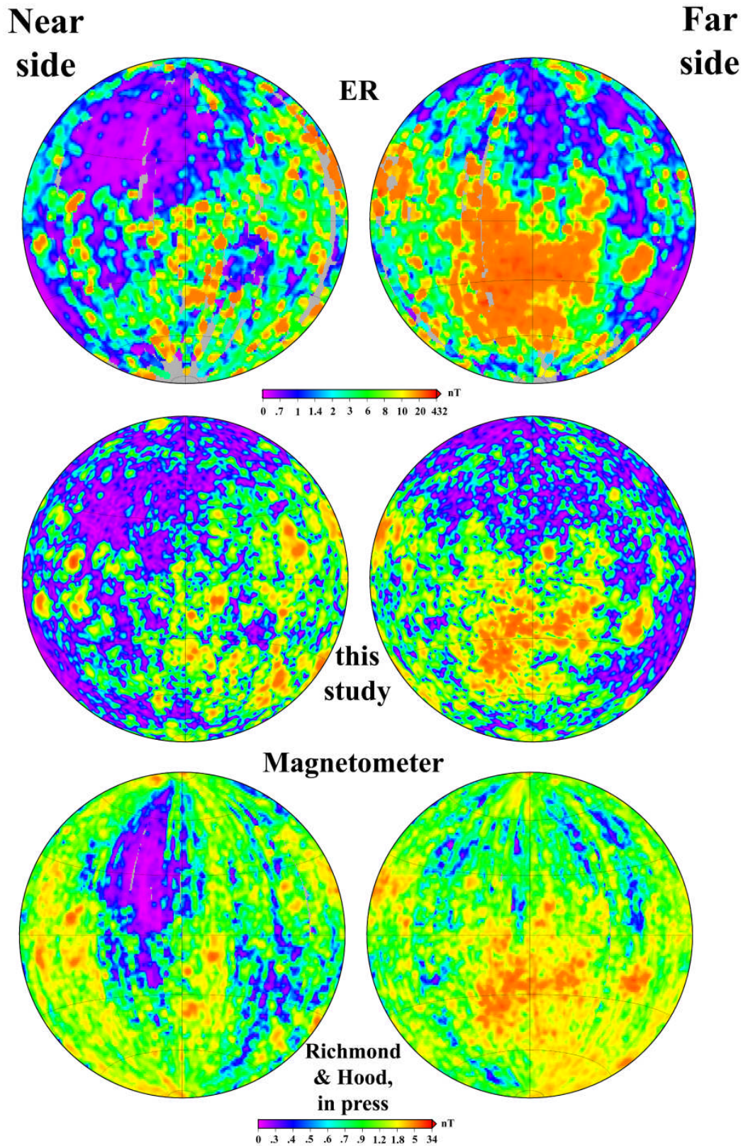
Figure 5, Purucker, Global lunar magnetic model
