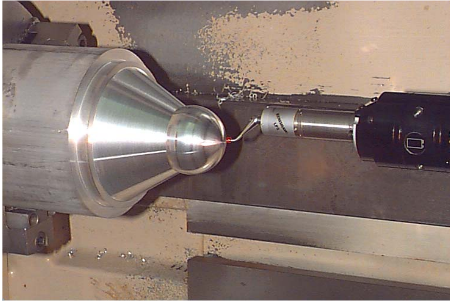
Figure 1: Probing Part Zero
