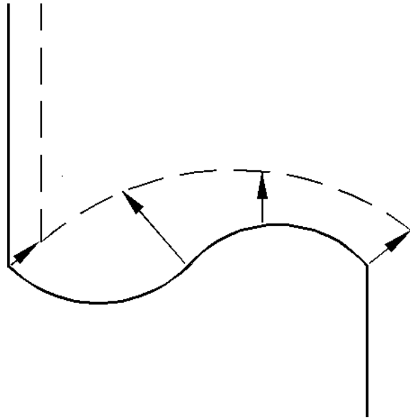
Figure 7: Curved Feature with Boundary Errors
