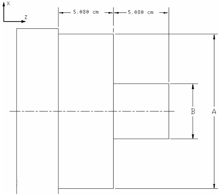
Figure 12: FACETST Part with Linear Features
