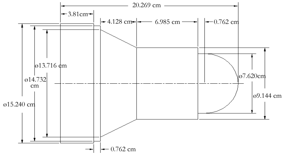
Figure 14: MODBAS2 Part with Cylinder, Taper and Dome Features.
