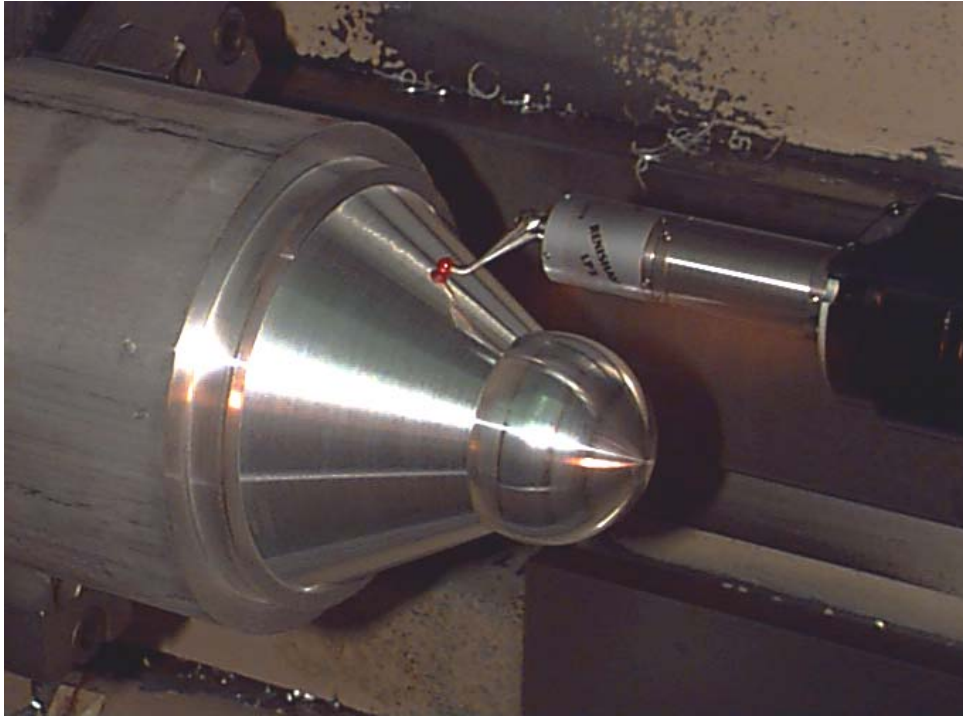
Figure 3: Probing the Taper
