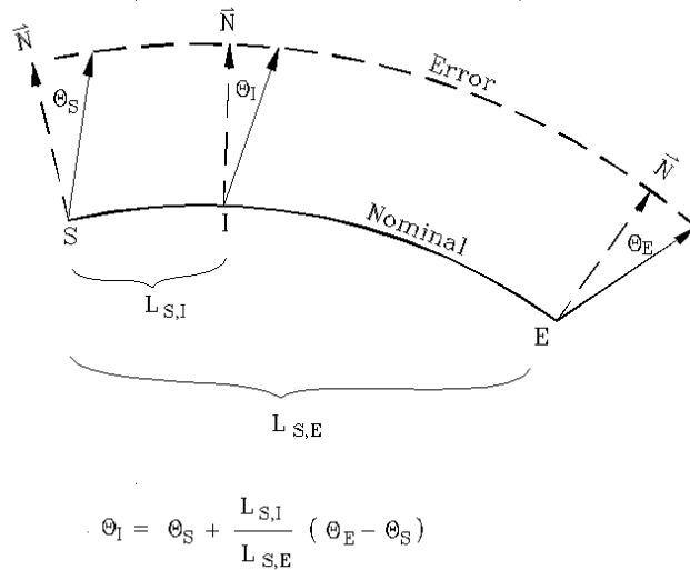
Figure 9: Mapping Nominal Points to Error Points.
