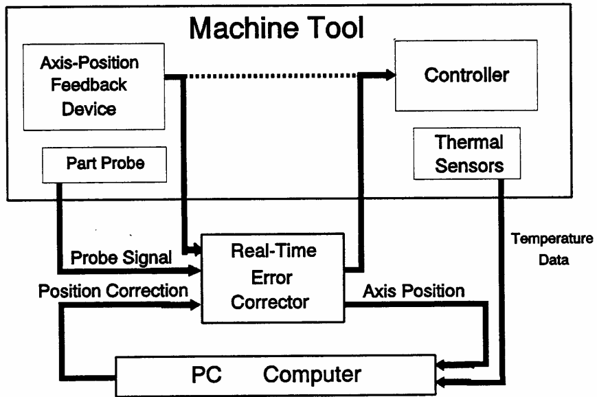
Figure 10: Error Compensation System
