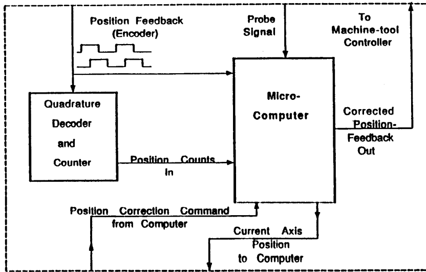
Figure 11: RTEC Architecture
