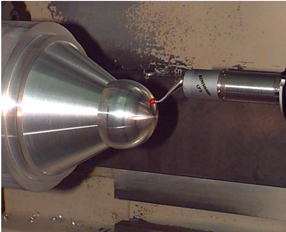
Figure 2: Probing Along the Dome
