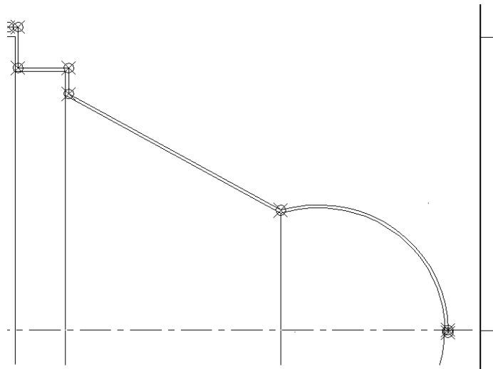
Figure 18: Semifinish and Finish Profiles for PIECS11
