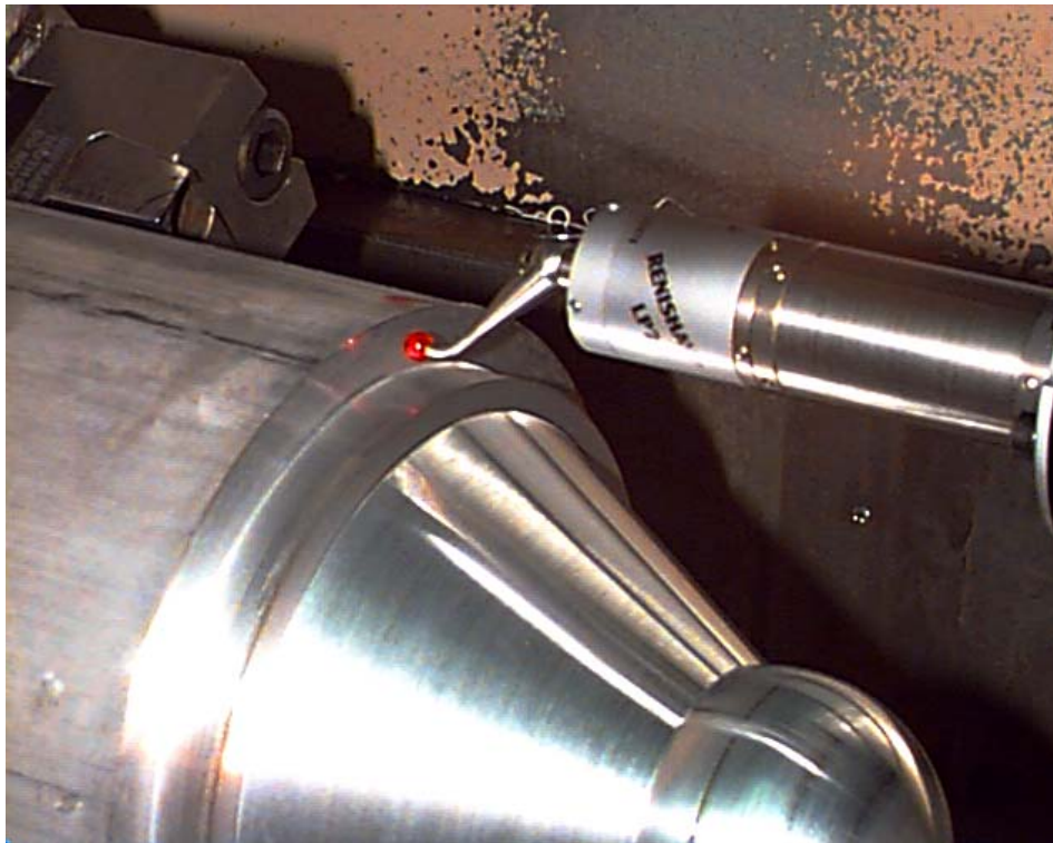
Figure 4: Probing the Base Plane
