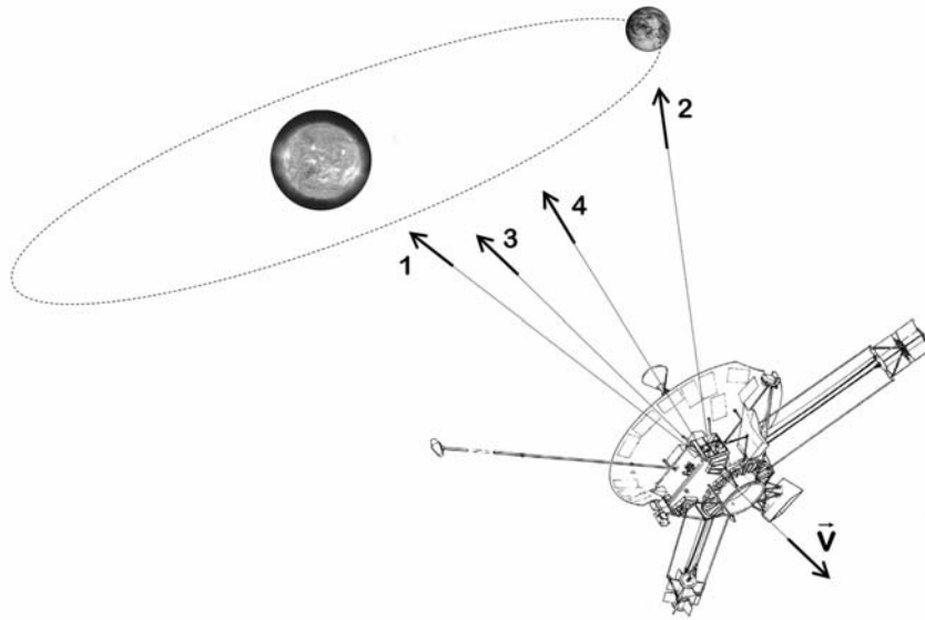
FIG. 4: Four possible directions for the anomalous acceleration acting on the Pioneer spacecraft: (1) towards the Sun, (2) towards the Earth, (3) along the direction of motion of the craft, or (4) along the spin axis.
