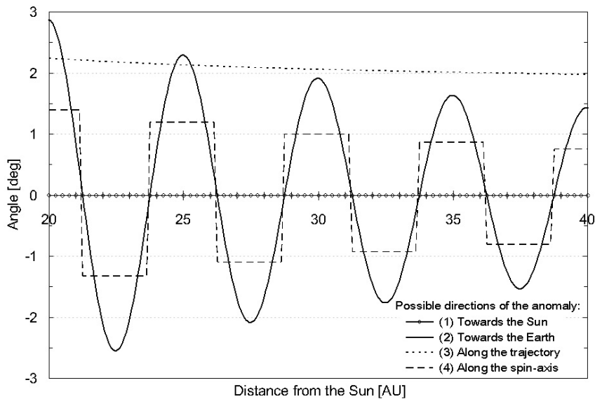
FIG. 5: The signatures for four possible directions of the anomalous acceleration acting on a deep-space craft. The signatures are distinctively different and are detectable with precise enough data and analysis.
