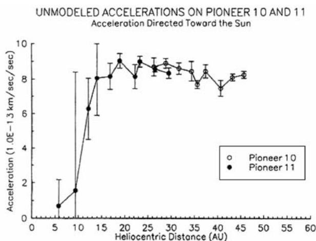
FIG. 3: An ODP plot of the early unmodeled accelerations of Pioneer 10 and Pioneer 11, from about 1981 to 1989 and 1977 to 1989, respectively.
