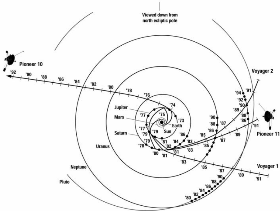
FIG. 2: Ecliptic pole view of Pioneer 10, Pioneer 11, and Voyager trajectories. Pioneer 11 is traveling approximately in the direction of the Sun’s orbital motion about the galactic center. The galactic center is approximately in the direction of the top of the figure.
