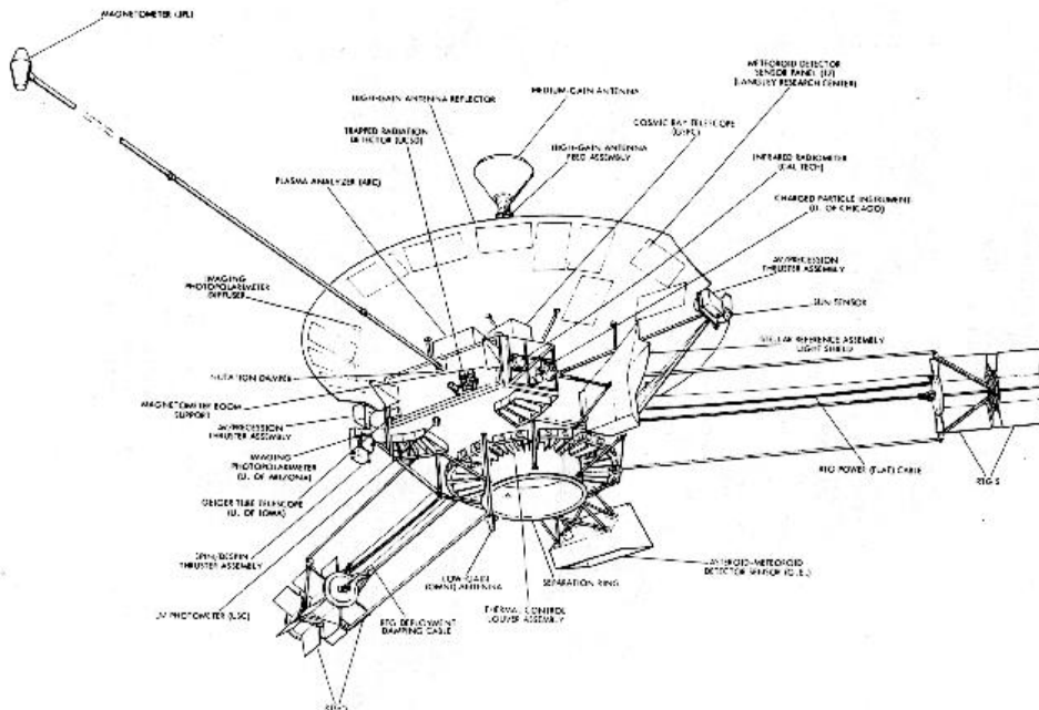
FIG. 1: A drawing of the Pioneer spacecraft.
