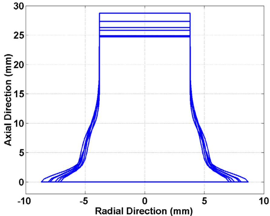
Figure 5. Six representative Taylor-test profiles for the steel cylinder predicted in a short Monte Carlo run in which there is a high degree of uncertainty in its plastic behavior. The variability in these profiles indicates the degree of their uncertainty arising from the uncertainties in the stress-strain curve for the material.
