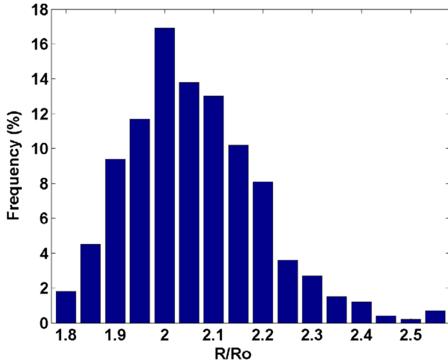
Figure 6. Histogram of the ratio of the radius at the base of the deformed cylinder to its initial value obtained from a Monte Carlo run of 1,000 simulations. This histogram represents the uncertainty in R/R_o coming from the assumed uncertainties in the plastic stress-strain behavior.
