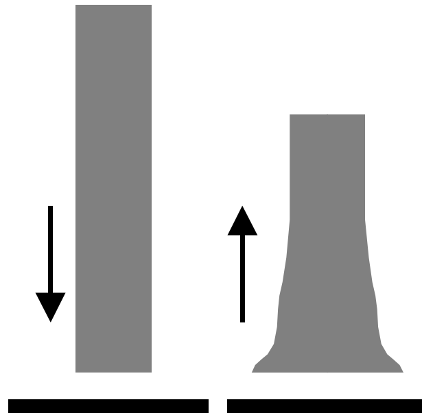
Figure 3. In the Taylor impact test, a cylinder is thrown with high velocity into a fixed, rigid plate (left) producing a significant permanent deformation in the rebounded cylinder (right).
