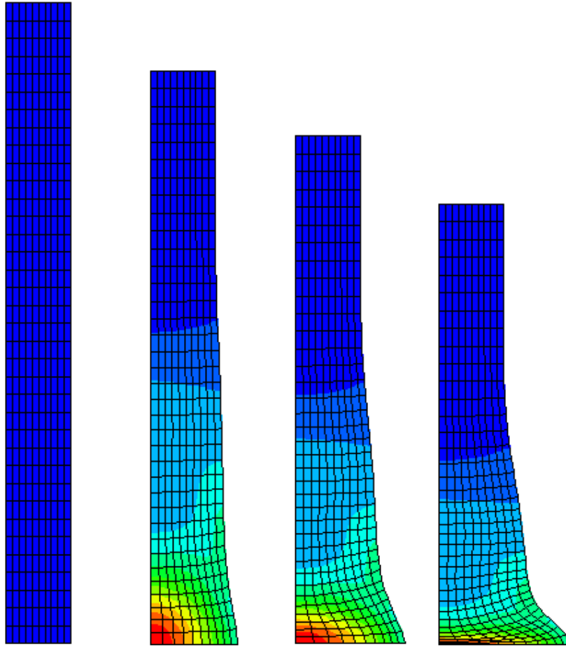
Figure 4. Simulation of the Taylor test described in the text. The figures show the half-cylinder shapes at times of 0 \mu\text{s} , 17 \mu\text{s} , 33 \mu\text{s} , and 50 \mu\text{s} after impact (from left to right). Their equivalent-strain patterns vary from 0% (dark blue) to maximum strains of 83%, 165%, and 248% (red) for the last three shapes, respectively.
