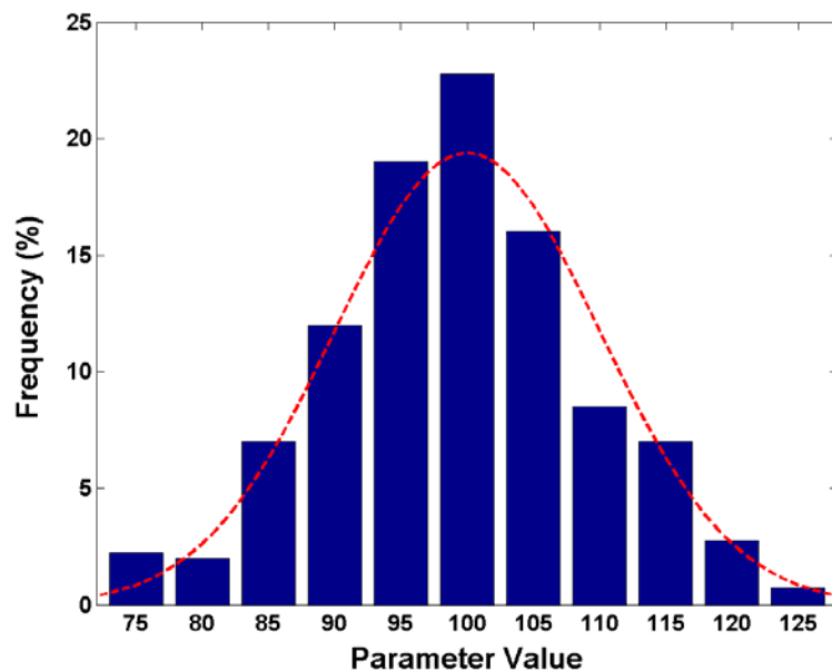
Figure 1. The frequency histogram of a set of 100 random numbers drawn from a normal pdf, shown as the dashed line.
