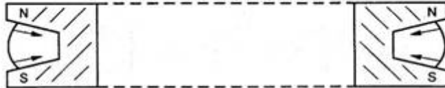
Figure 3.3. Cross section of weak focusing circular accelerator.
