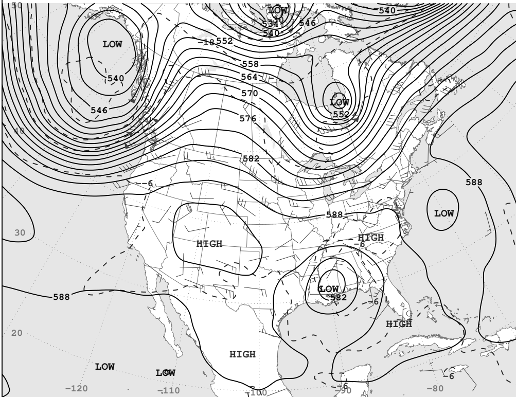
SUN, AUG 24, 2008 500-Millibar Height Contours at 7:00 A.M. E.S.T.
