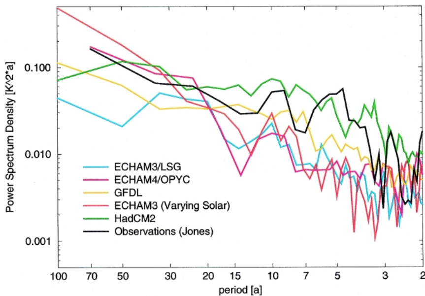
FIG. 3. Power spectra of global-mean, annual temperatures from a number of coupled model control integrations compared with that derived from observations. The model designators are explained in Table 3. The record lengths vary and so do the confidence limits. In most cases, the confidence limits are large compared to differences between spectra. Note the difference in energy in the 30–50-yr band, where most detection work is done, is of order 2–4. See Stouffer et al. 1999 for additional details.
