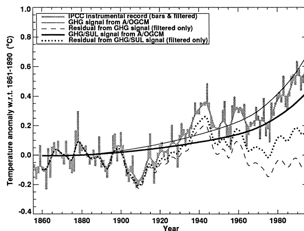
FIG. 1. Annual-mean observed global temperatures (expressed as anomalies from 1861 to 1890) for 1856–1995 (gray histogram and 10-yr Gaussian filter). The thick and thin smooth lines, respectively, are the anthropogenic and greenhouse-gas-only fitted responses (from Jones and Hegerl 1998). The model responses come from Hegerl et al. 1997. The dotted and dashed lines, respectively, are the “residuals” after extracting the anthropogenic and greenhouse-gas-only signals from the 10-yr Gaussian smoothed data.
