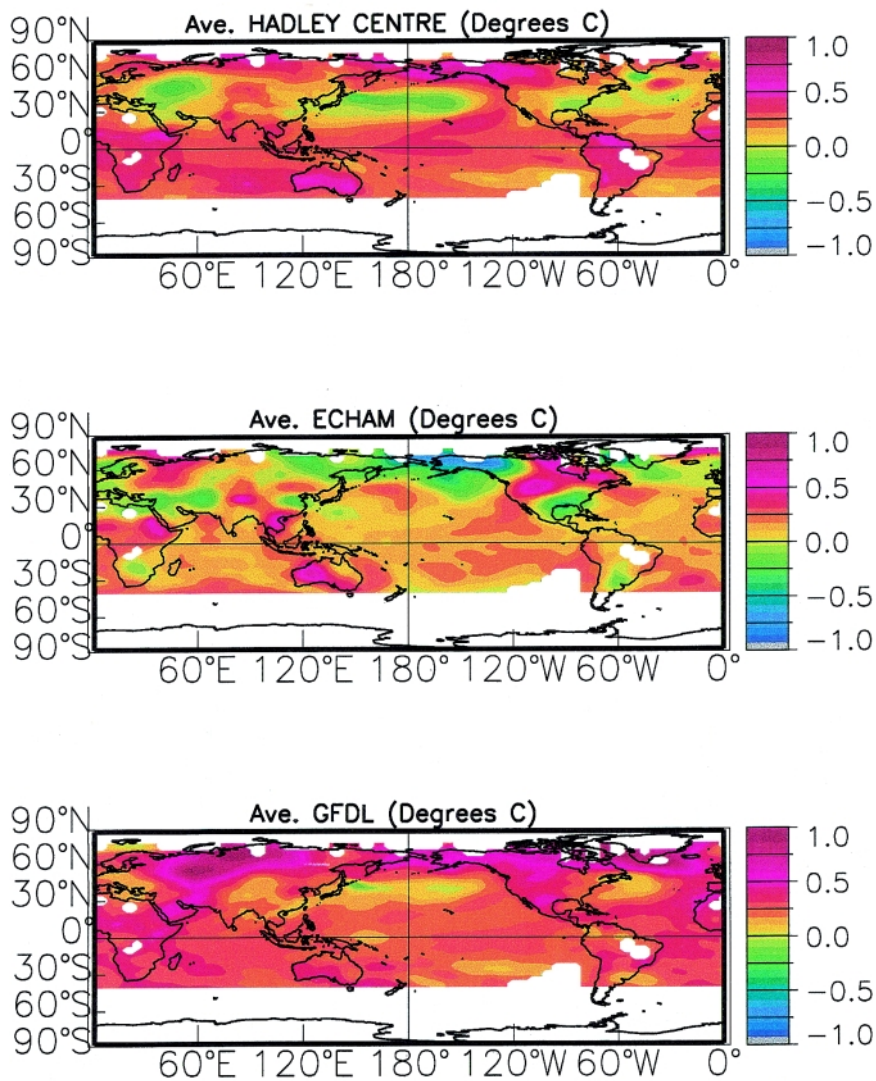
FIG. 7. Changes in smoothed near-surface temperature (°C) between 1945 and 1995 produced by ensemble averages from coupled global climate models of the HadCM2, MPI, and GFDL. All models were forced by their own independent estimates of an anthropogenic signal composed of greenhouse gases and direct sulfate aerosol effects.
