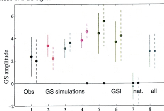
b) Attribution diagram for the greenhouse gas signal only
