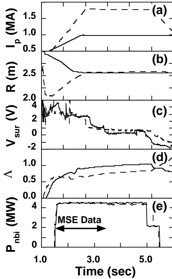
Figure 5. Time evolution of plasma current I_p , major radius R , \Delta \equiv \beta_{pol} + \ell_i/2 , surface voltage V_{sur} , and neutral beam heating power P_{nbi} , for two discharges with different plasma currents.
