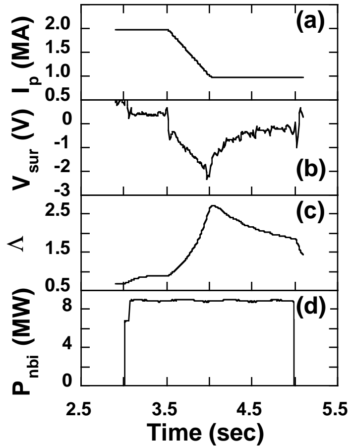
Figure 1. Time evolution of plasma current I_p , surface voltage V_{sur} , \Lambda \equiv \beta_{pol} + \ell_i/2 , and neutral beam heating power P_{nbi} , for a discharge with a -2.0 MA/sec current ramp at 3.5 sec. The plasma major radius was R = 2.45 m.
