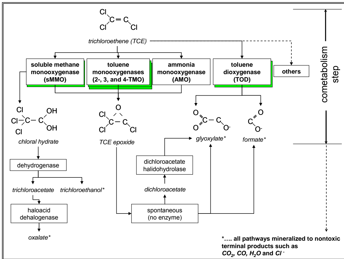
Figure 1. Some of the cometabolic pathways for TCE (this figure represents a compilation of pathways documented in the University of Minnesota Biocatalysis/Biodegradation Database, http://umbbd.msi.umn.edu/ ) Existing EAP assays available for the highlighted items
