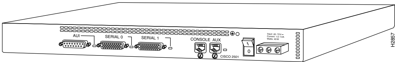
Figure 1-3 Configurations for Models 2501-DC and 2503-DC Multiprotocol Routers
