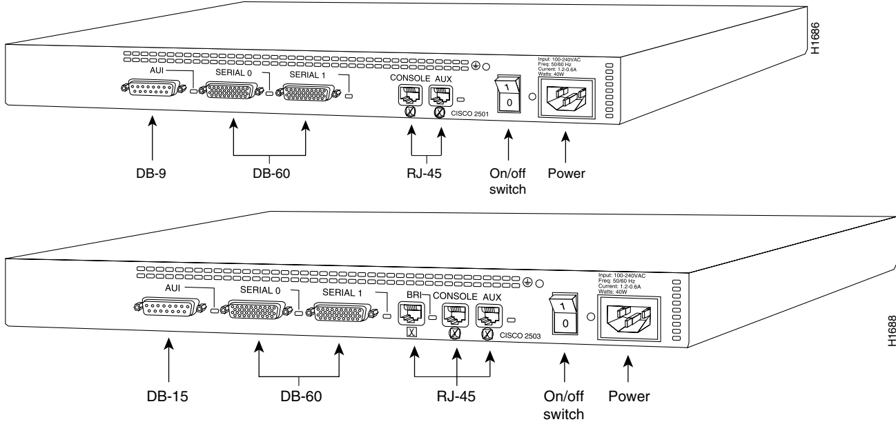
Figure 1-2 Configurations for Models 2501 and 2503 Multiprotocol Routers
