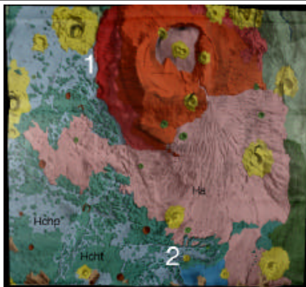
Figure 1: Regional geologic map of Apollinaris Patera region based on geologic map by Scott et al.
